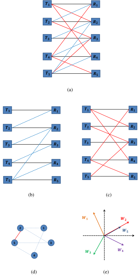
Fig. 2: (a) 5-user interference channel; (b) The TIN component; (c) The TIM component; (d) The alignment graph (red solid lines) for the TIM component showing conflicts as dashed blue lines; (e) An achievable scheme to achieve symmetric GDoF of 0.3.
