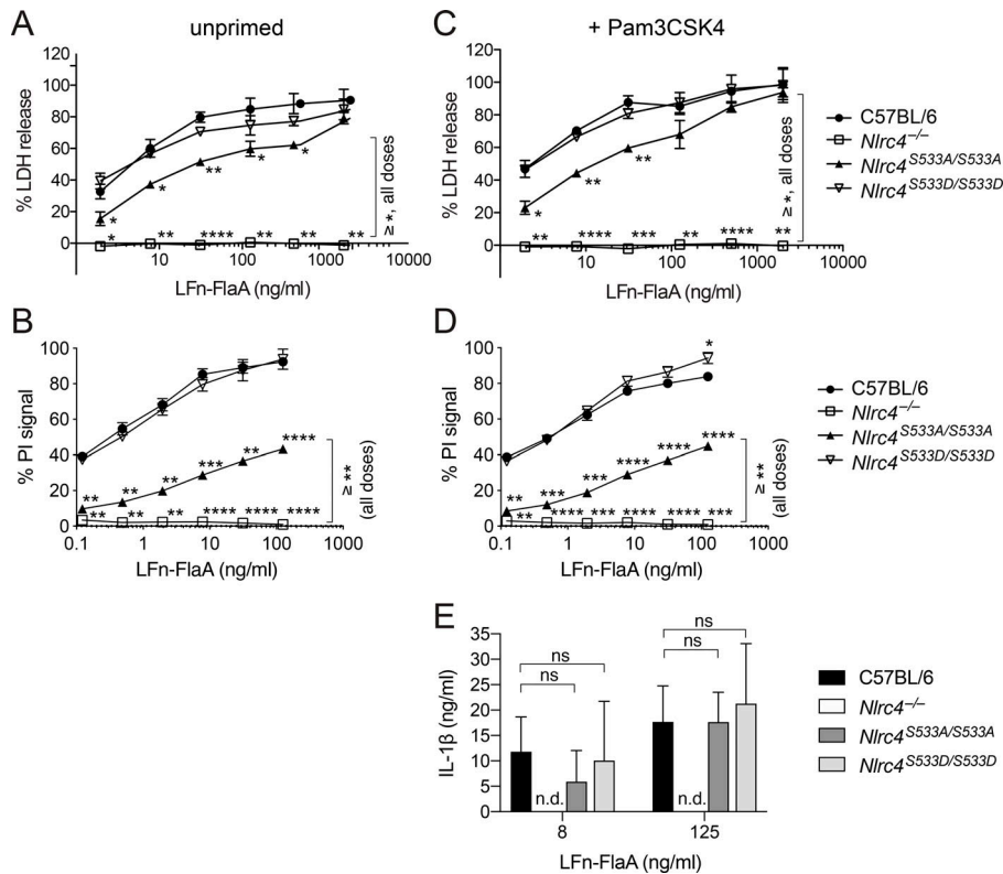
Figure 2. NLRC4 phosphorylation is neither sufficient nor strictly required for response to cytosolic flagellin. (A–E) Macrophages were either left unprimed (A and B) or primed 4 h with 1 μg/ml Pam3CSK4 (C–E) and then treated with 4 μg/ml PA and the indicated dose of LFn-FlaA to activate NLRC4. LDH release (A and C), PI uptake (B and D), or IL-1β release (E) was measured after 4 h. All data are representative of three independent experiments (three biological replicates per experiment). Mean ± SD; n.d., not detectable. Repeated measures two-way ANOVA with Dunnett’s multiple comparisons post-test, all genotypes vs. C57BL/6J (or Nlrc4 S533A/S533A vs. Nlrc4 -/- as indicated), *, P < 0.05, **, P < 0.005, ***, P < 0.0005, ****, P < 0.00001; ns, not significant.
