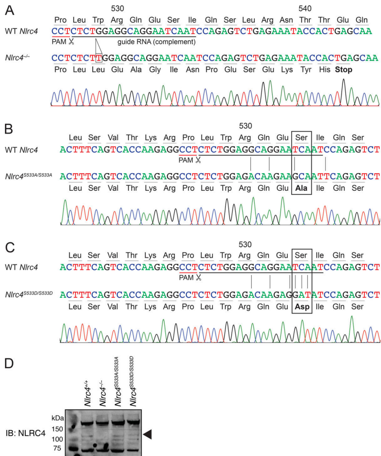
Figure 1. CRISPR/Cas9 targeting of Nlrc4 . (A–C) The sequence of the Nlrc4 locus in WT C57BL/6J compared with CRISPR/Cas9-generated (A) Nlrc4 -/- , (B) Nlrc4 S533A/S533A , and (C) Nlrc4 S533D/S533D mice. Sanger sequences traces are shown for mutant mice. Guide RNA sequence and protospacer-adjacent motif (PAM) for CRISPR/Cas9 targeting, as well as nonsilent base exchanges, are indicated. (D) Immunoblot (IB) of NLRC4 levels in bone marrow–derived macrophages. Representative of two independent experiments.
