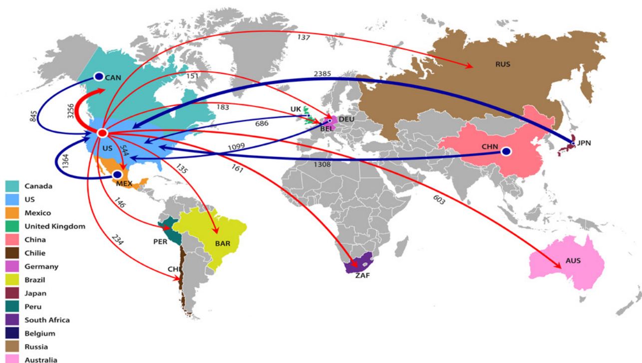
Figure 10. Top flows of CO 2 emissions embodied in the U.S. import and export of construction machinery (NAICS 333120) in 2018 (kt CO 2 )
