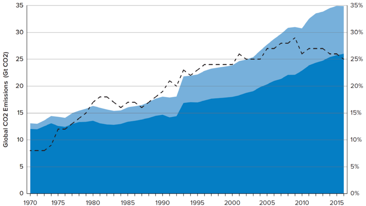
Figure 1. Global CO 2 emissions and proportion embodied in trade (Hasanbeigi et al. 2018)
