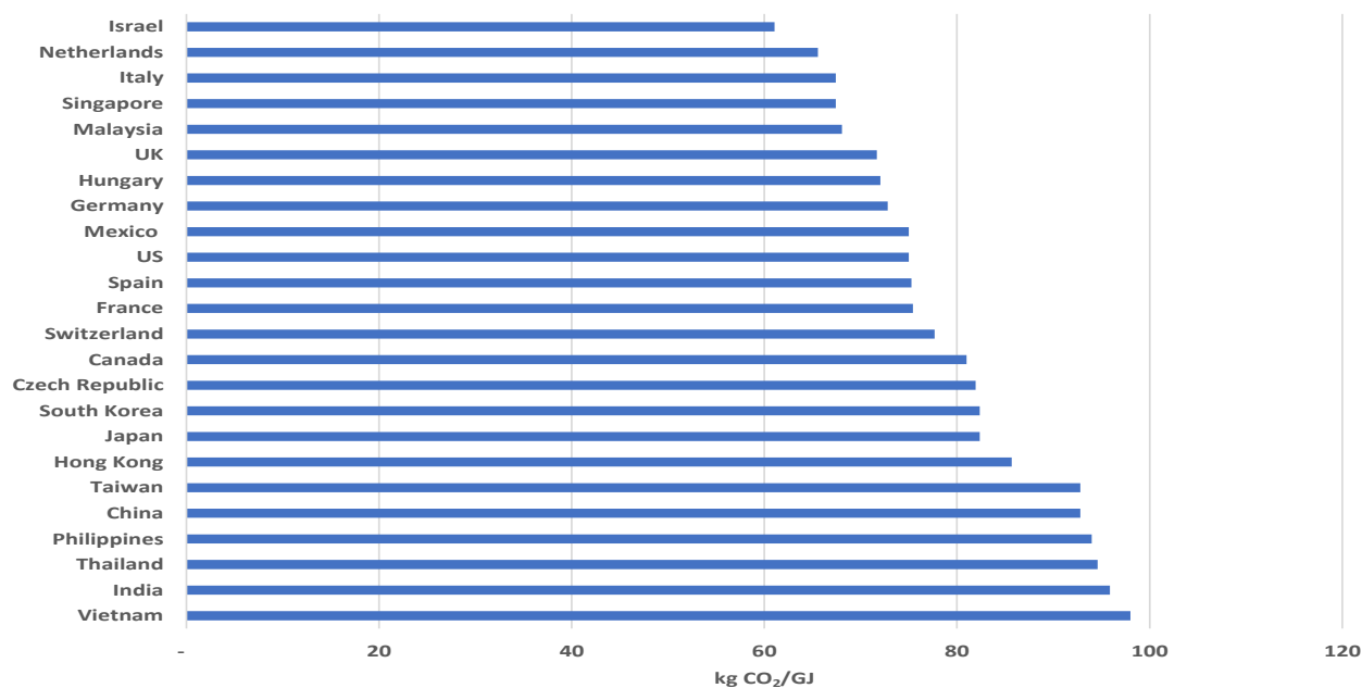
Figure 4. Weighted Average CO 2 emissions factor of fuels used in industry in selected countries in 2017 (kg CO 2 /GJ)
