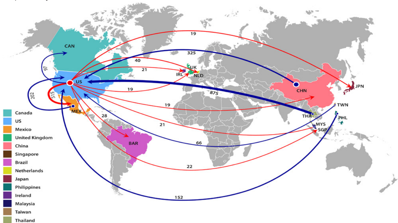
Figure 6. Top flows of CO 2 emissions embodied in the U.S. import and export of Computer Storage Devices (NAICS 334112) in 2018 (kt CO 2 )
