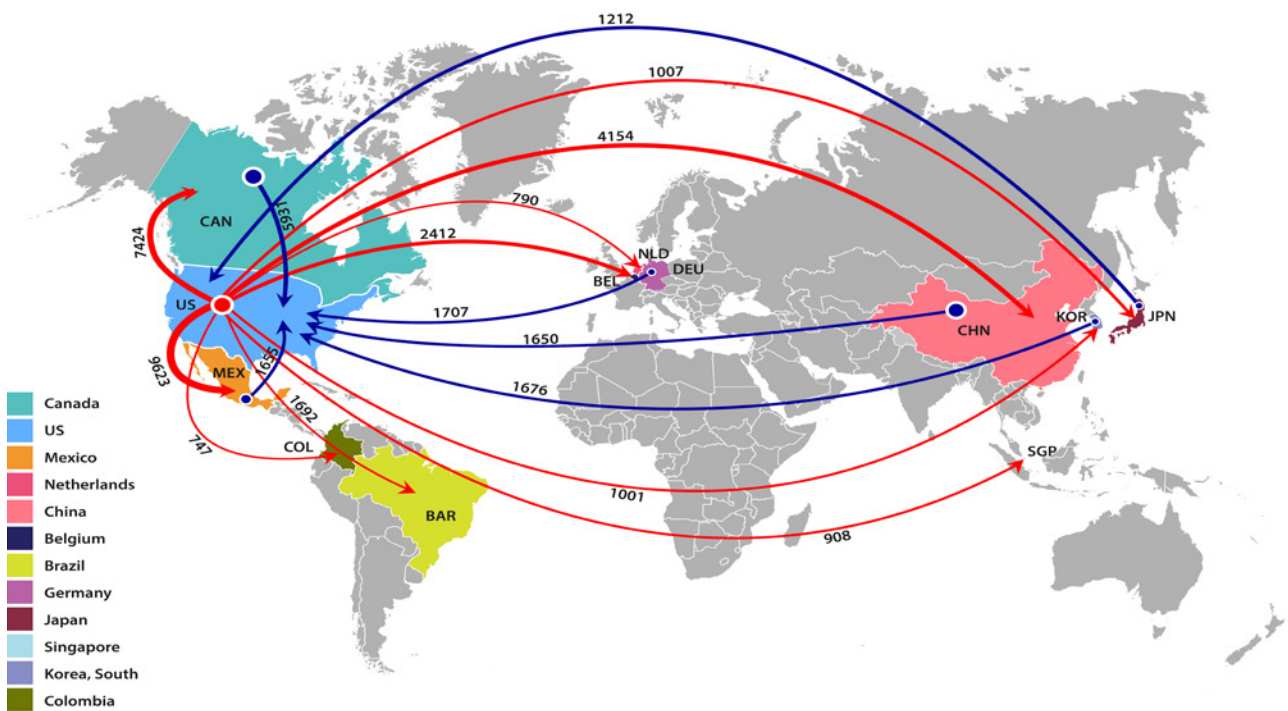
Figure 13. Top flows of CO 2 emissions embodied in the U.S. import and export of plastics materials and resins (NAICS 325211) in 2018 (kt CO 2 )
