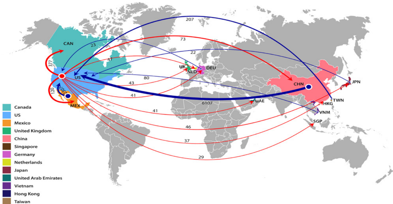
Figure 5. Top flows of CO 2 emissions embodied in the U.S. import and export of Electronic Computers (NAICS 334111) in 2018 (kt CO 2 )
