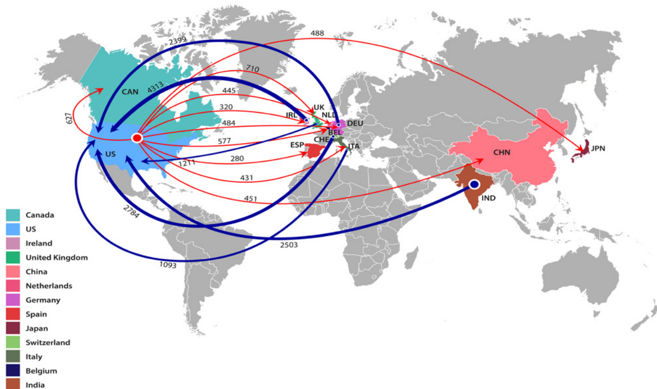
Figure 12. Top flows of CO 2 emissions embodied in the U.S. import and export of pharmaceutical preparations products (NAICS 325412) in 2018 (kt CO 2 )
