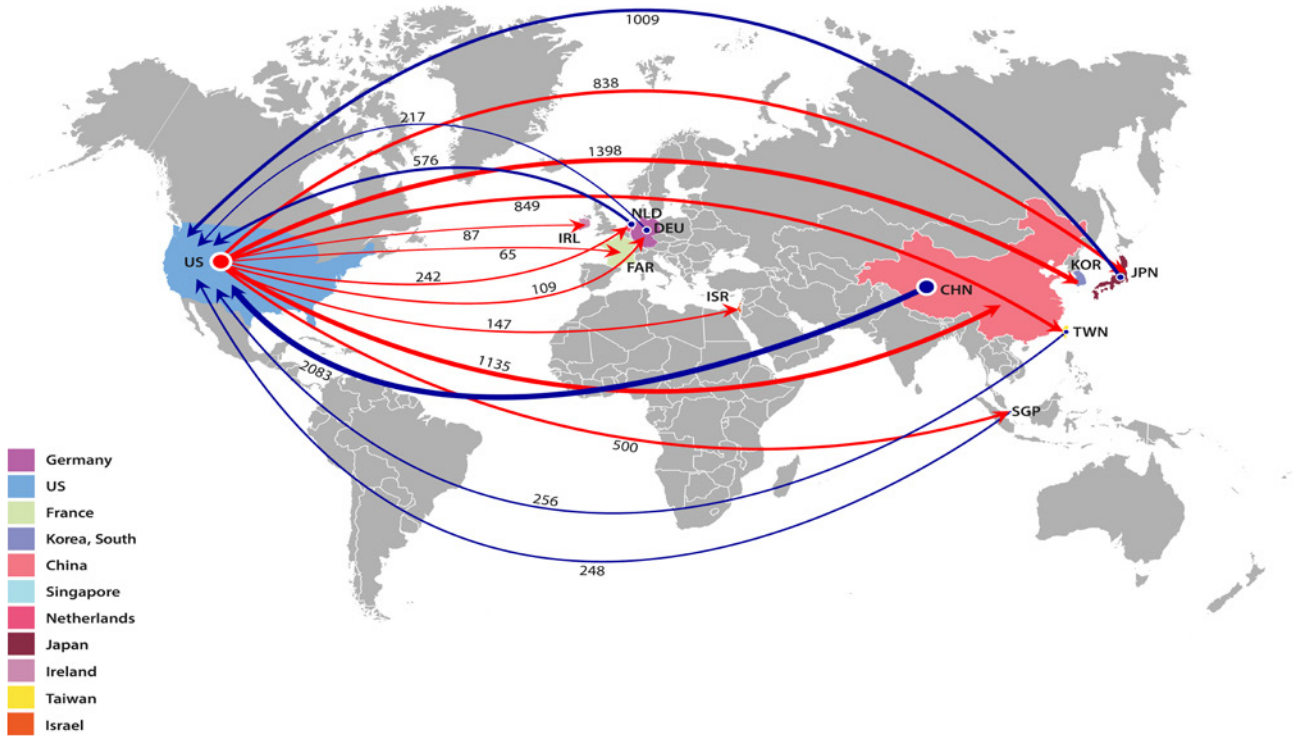
Figure 11. Top flows of CO 2 emissions embodied in the U.S. import and export of semiconductors machinery (NAICS 333242) in 2018 (kt CO 2 )
