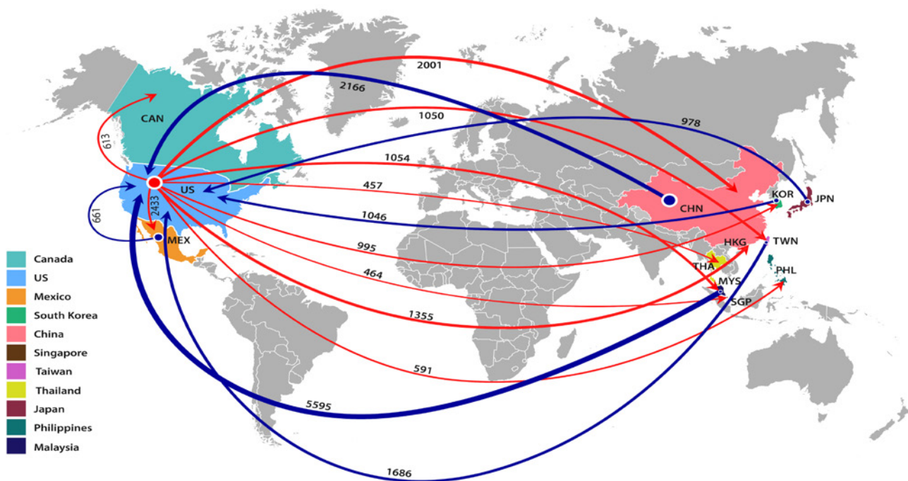
Figure 7. Top flows of CO 2 emissions embodied in the U.S. import and export of Semiconductors (NAICS 334413) in 2018 (kt CO 2 )
