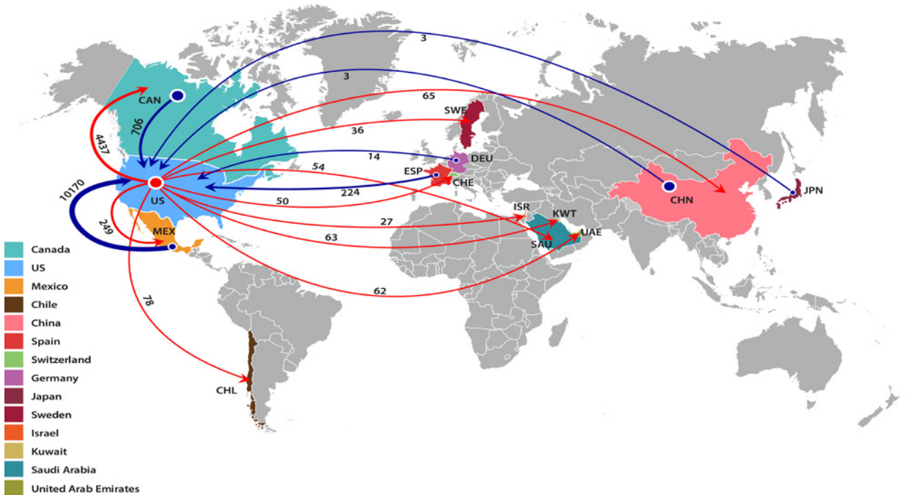
Figure 9. Top flows of CO 2 emissions embodied in the U.S. import and export of light truck and utility vehicle (NAICS 336112) in 2018 (kt CO 2 )
