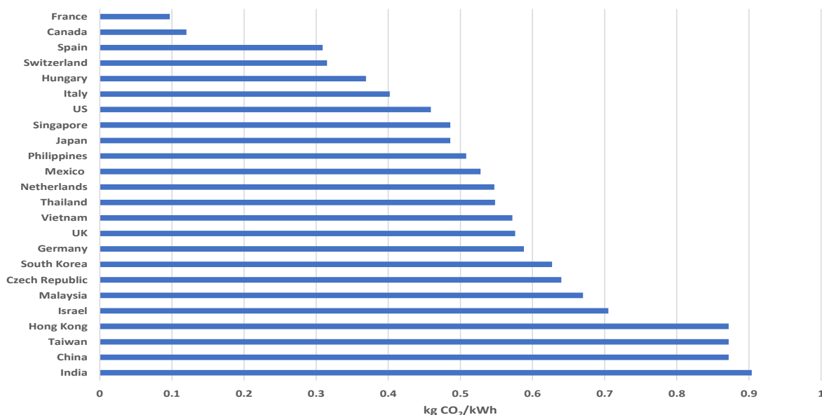
Figure 3. Electricity grid CO 2 emissions factor in selected countries in 2017 (kg CO 2 /kWh)
