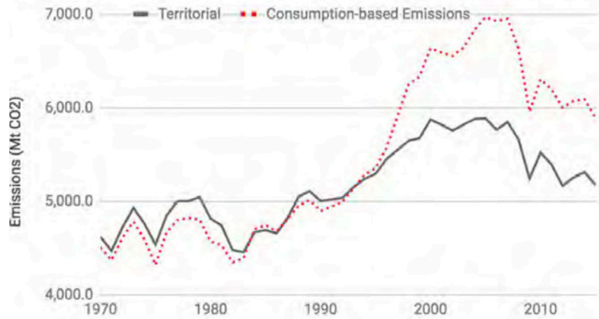
Figure 2. Territorial and consumption-based emissions in the U.S. 1970-2015 (Hasanbeigi et al. 2018)
