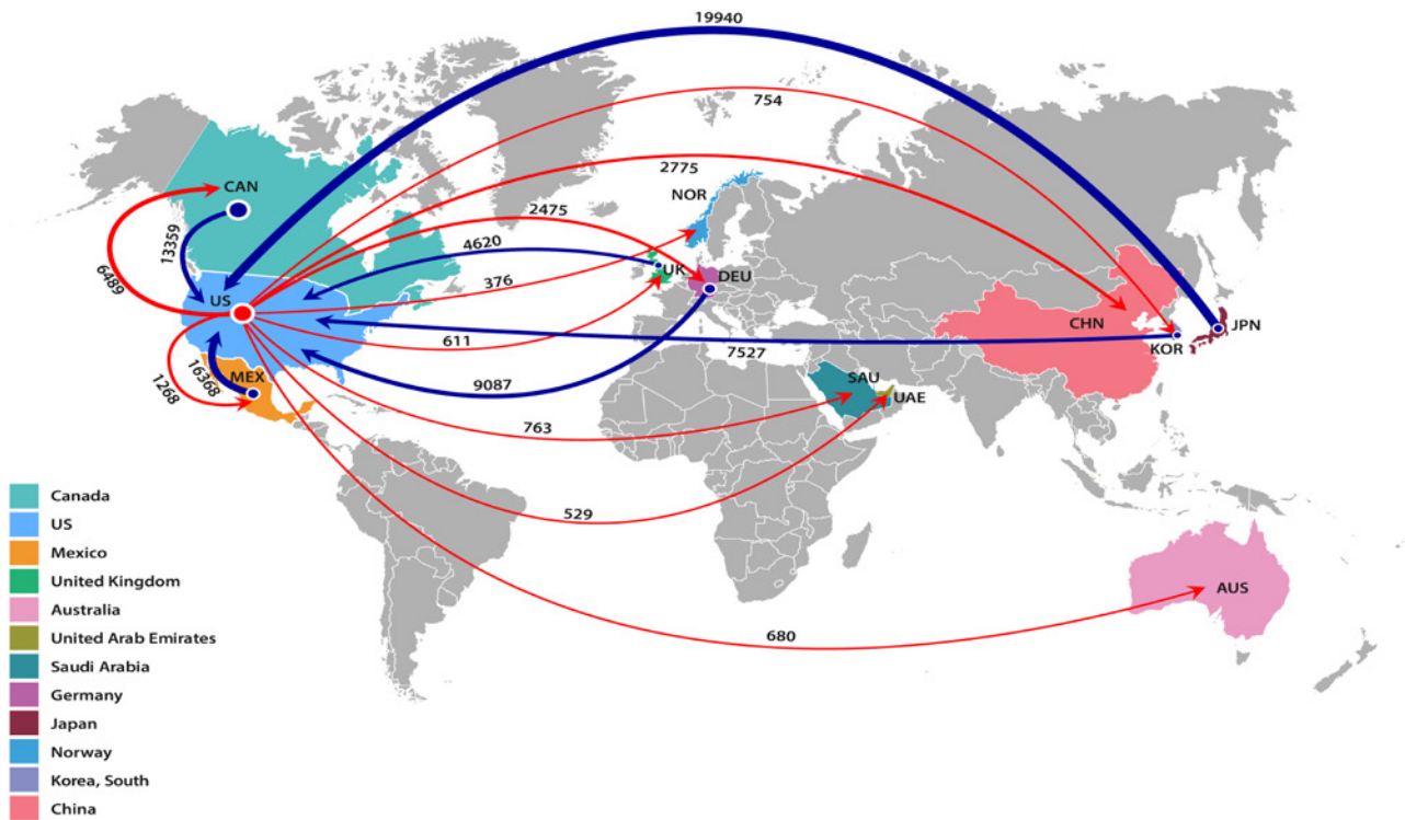
Figure 8. Top flows of CO 2 emissions embodied in the U.S. import and export of autos and light duty motor vehicles (NAICS 336111) in 2018 (kt CO 2 )
