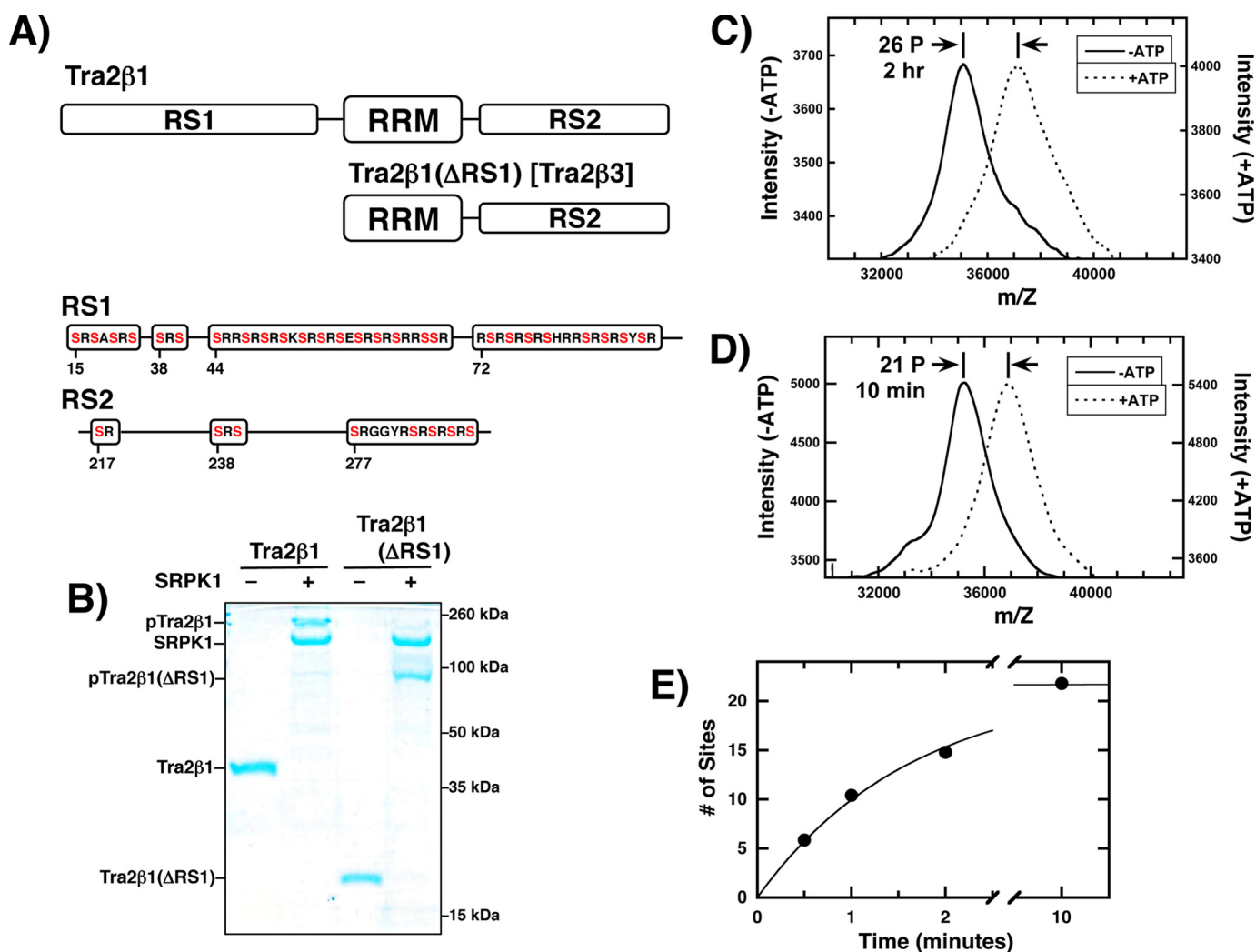
FIGURE 2. Tra2 \beta 1 phosphorylation by SRPK1. A, RS domains (RS1 and RS2) in Tra2 \beta 1 and Tra2 \beta 1( \Delta RS1). B, Phos-tag SDS-PAGE of Tra2 \beta 1 and Tra2 \beta 1( \Delta RS1) with and without SRPK1 phosphorylation. C and D, MALDI-TOF of Tra2 \beta 1 with SRPK1 after 10 min (C) and 2 h (D) of incubation with ATP. The molecular mass of Tra2 \beta 1 increases by 1.64 and 2.05 kDa after 10-min and 2-h incubations. E, SRPK1 phosphorylation of Tra2 \beta 1 by autoradiography. Data were fit to a rate constant of 0.6 min -1 and 21 total sites.
