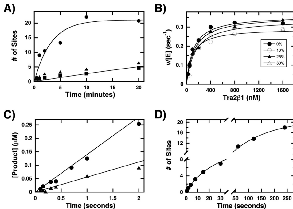
FIGURE 3. Kinetic analysis of Tra2 \beta 1. A , start-trap experiment. SRPK1 (1 \mu M) and Tra2 \beta 1 (0.2 \mu M) are pre-equilibrated before addition of ATP (50 \mu M) in the absence (●) and presence (▲) of kdSRPK1 (60 \mu M). The data in the absence of kdSRPK1 are fit to a rate constant of 0.31 min -1 and an end point of 21 sites. A control reaction is run by pre-equilibrating SRPK1, kdSRPK1, and Tra2 \beta 1 prior to ATP addition (■) and fit to a slope of 0.29 sites/min. B , viscosity experiments. Initial velocity of SRPK1 is measured as a function of Tra2 \beta 1 at varying amounts of sucrose. The data at 0% sucrose are displayed in Table 1. C , rapid quench flow experiments. Tra2 \beta 1 (3 \mu M) is pre-equilibrated with 0.2 (▲) and 0.5 \mu M (●) SRPK1 and then reacted with 50 \mu M ATP. The data are fit to slopes of 0.06 and 0.14 \mu M/s at 0.2 and 0.5 \mu M SRPK1. D , single turnover experiment. SRPK1 (2 \mu M), Tra2 \beta 1 (0.4 \mu M), and ATP (100 \mu M) are reacted in the rapid quench flow instrument, and the number of sites are plotted with time (0.1–240 s). The data are fit to a double exponential with amplitudes and rate constants of 5.0 and 16 sites and 0.075 and 0.0065 s -1 .
