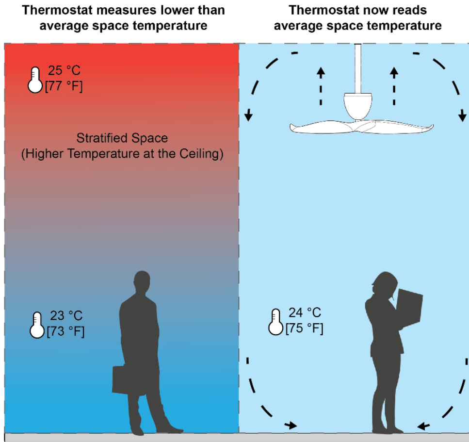
Figure 5. Ceiling fans (blowing upwards) for destratification.
