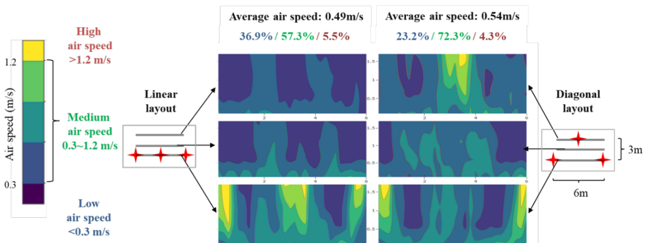
Figure S4 Air speed distribution for linear and diagonal ceiling fans operation layout.
