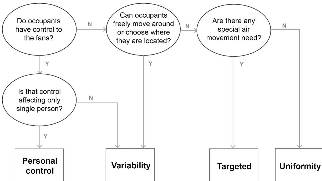
Figure T5. Flow chart of design intent for air speed and distribution.
