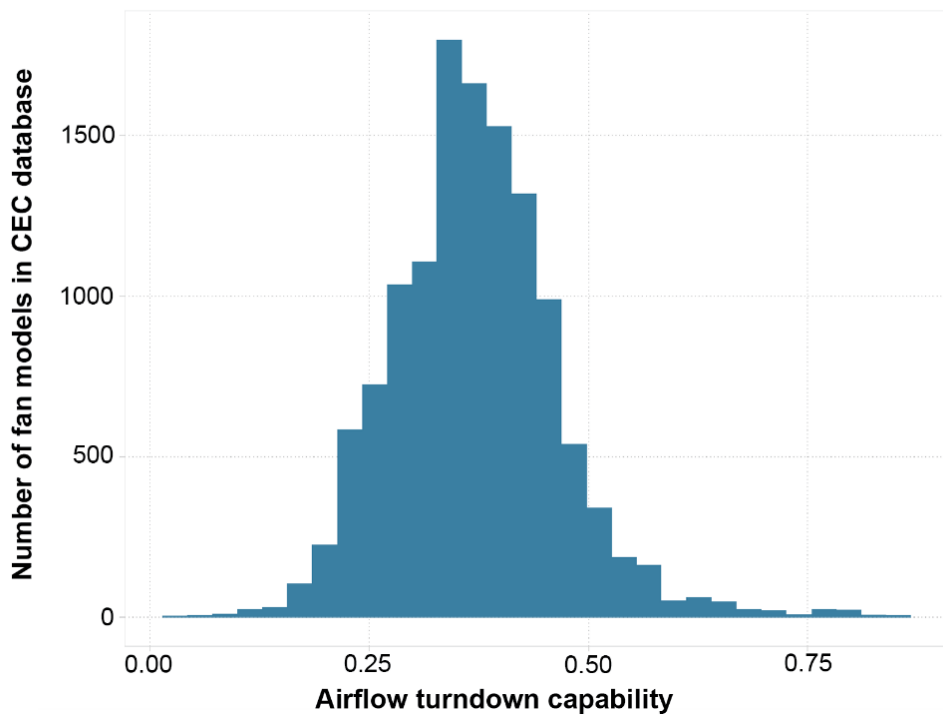
Figure 14. Minimum fan speed for ceiling fans in the CEC MAEDbS database.
