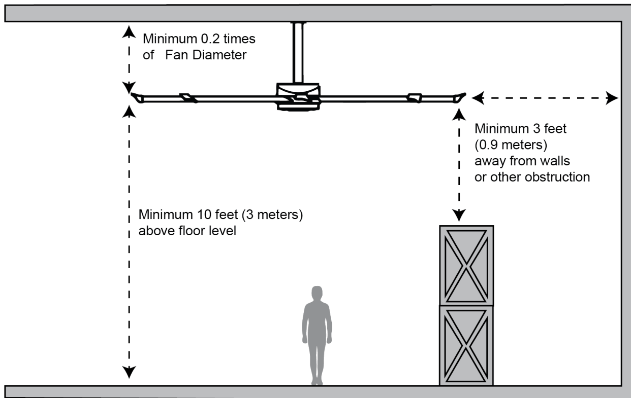
Figure 38. Minimum clearances for large diameter ceiling fans.
