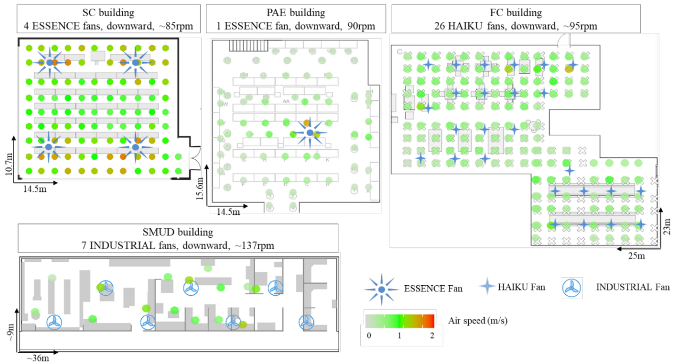
Figure S1. Floor plan and air speed distribution in the 4 tested buildings. The magnitude of air speed at each site is averaged by heights.
