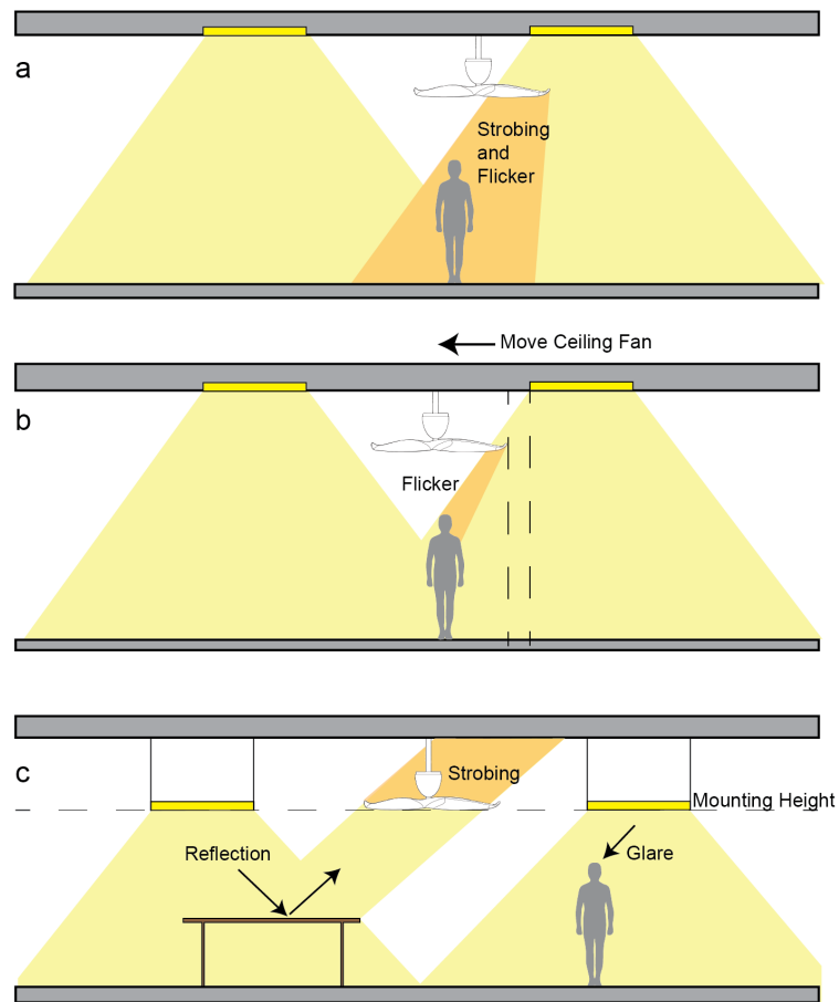
Figure T9. Sectional illustrations on the interactions between ceiling fans and lighting fixtures across different configurations: (a) strobbing and flicker, (b) flicker, and (c) ceiling strobing.
