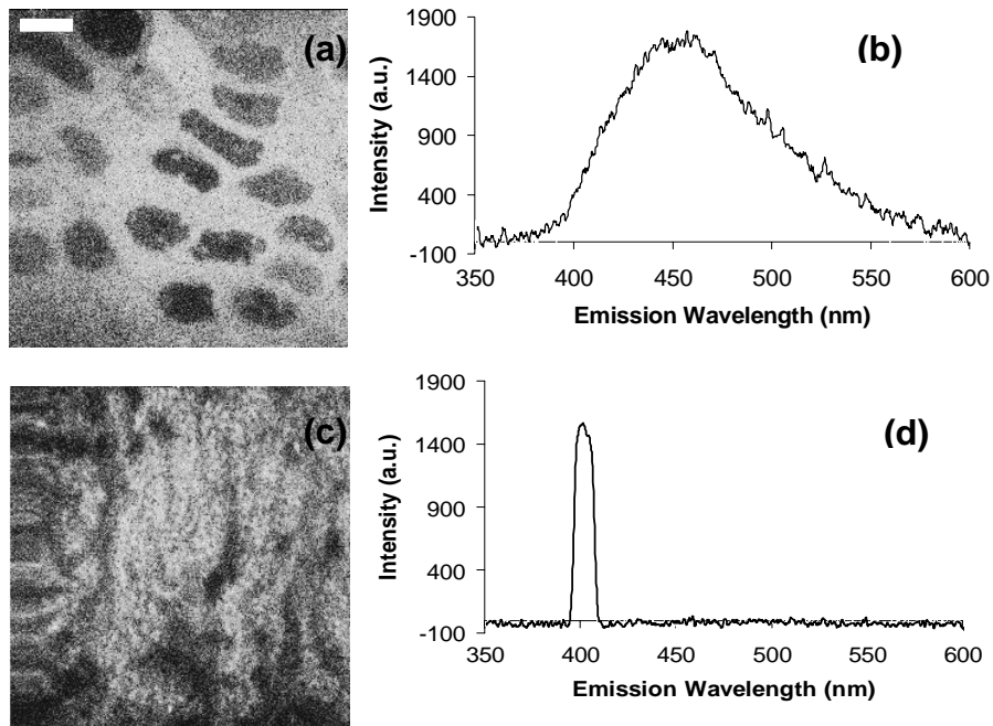
Fig. 5. Origin of signals in two-photon microscopy of the rabbit cornea. (a) Two-photon image of the corneal epithelium for \lambda_{ex}=750\text{nm} ; and the corresponding emission spectrum (b) consisting of cellular TPEF signal. (c) Two-photon image of the corneal stroma for \lambda_{ex}=800\text{nm} ; and the corresponding emission spectrum (d) consisting of SHG signal from collagen. Spectra acquisition time, \Delta t=60\text{s} . Scale bar is 6\mu\text{m} .
