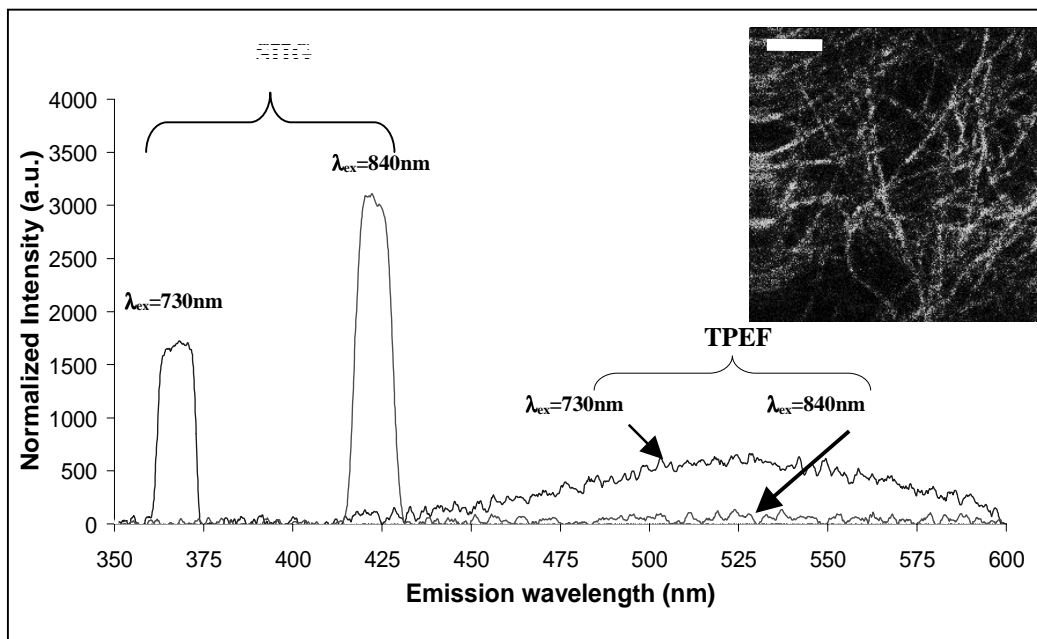
Fig. 1. Emission spectra for RAFT collagen for \lambda_{ex}=730 , and 840nm at z=0\mu\text{m} for acquisition time \Delta t=60\text{s} . Inset shows two-photon image of collagen for \lambda_{ex}=840\text{nm} at z=0\mu\text{m} . Scale bar is 7\mu\text{m} .
