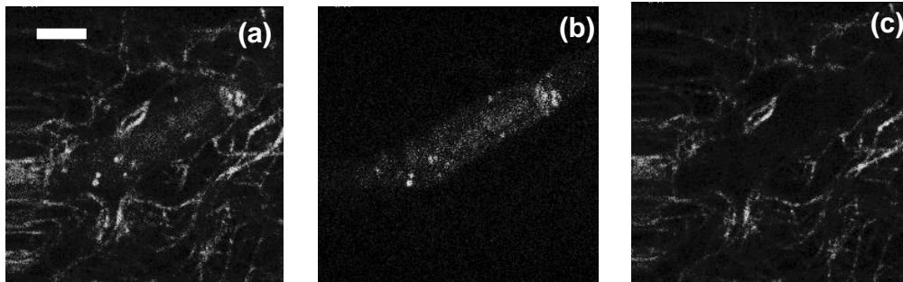
Fig. 6. Two-photon images of the same site in the RAFT acquired for \lambda_{ex}=840\text{nm} , at z=80\mu\text{m} , using three different emission filters in front of the PMT: (a) an SBG39 emission filter (320-600nm); (b) a 520/40nm band-pass filter; and (c) a 440/40nm band-pass filter. Scale bar is 6\mu\text{m} .
