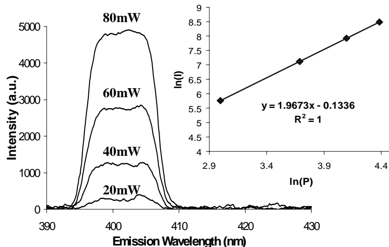
Fig. 2. Emission spectra from RAFT collagen for powers entering the microscope, P = 20, 40, 60, and 80\text{mW} , \lambda_{\text{ex}}=800\text{nm} , z=0\mu\text{m} . Spectra acquisition time was \Delta t=60\text{s} . Inset shows a plot of the natural logarithm of the SHG intensity as a function of the natural logarithm of the excitation power.
