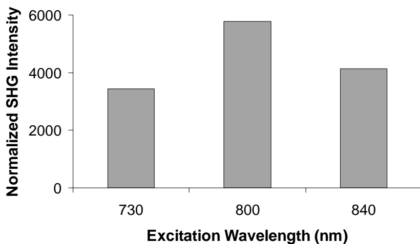
Fig. 3. Spectral dependence of reflected SHG intensity.
