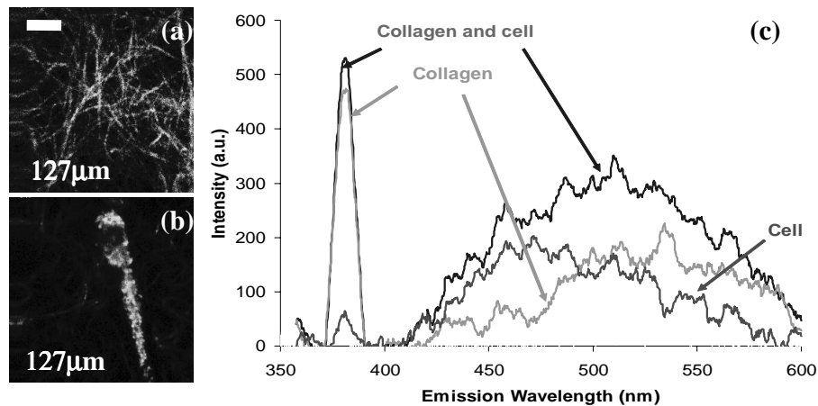
Fig. 4. Two-photon images from RAFT collagen only (a) and for collagen and cell (b) for \lambda_{\text{ex}}=750\text{nm} , P=57.3\text{mW} , z=127\mu\text{m} . Scale bar is 7\mu\text{m} . The corresponding emission spectra ( \Delta t=60\text{s} ) are shown in (c).
