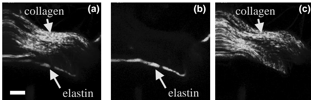
Fig. 7. Spectral filtering of the collagen and elastin components of the rabbit aortic wall for \lambda_{\text{ex}}=800\text{nm} . (a) Two-photon image of the rabbit aorta acquired with an SBG39 emission filter (320-600nm); (b) two-photon image from the same sample site as in (a) acquired with a 520/40nm band-pass emission filter; (c) two-photon image from the same sample site as in (a) acquired with a 400/10nm band-pass emission filter. Scale bar is 5 \mu\text{m} .
