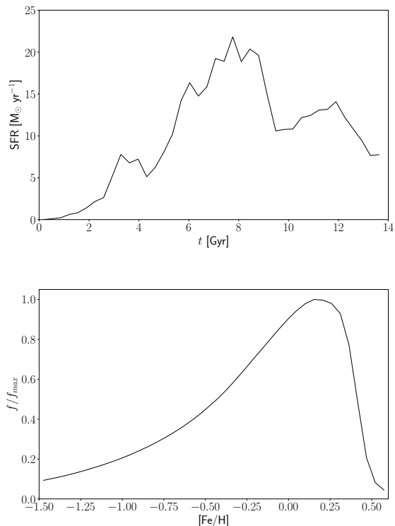
Figure 3. Top: The star formation history of the model. The initial star formation rate is very low but it rises rapidly to a peak at \sim 8 Gyr. Bottom: The metallicity distribution function over the entire galaxy.
