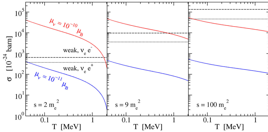
FIG. 1 (color online). The weak and magnetic scattering cross sections as a function of temperature for different values of the invariant variable s . The weak cross sections for \nu_e - e^- and \nu_e - e^+ scattering are represented by the black dashed and black dotted lines respectively. The magnetic cross sections for neutrino-electron (or positron) scattering are shown as the solid lines for two possible effective magnetic moments (red— 10^{-10}\mu_B and blue— 10^{-11}\mu_B ).
