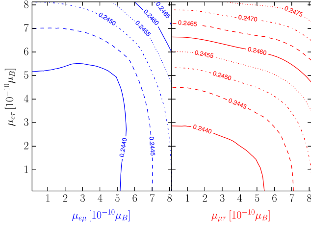
FIG. 7 (color online). Contours of constant Y_P in the \mu_{e\tau} versus \mu_{e\mu} (left) or \mu_{\mu\tau} (right) planes. The third transition magnetic moment is set to be \sim 10^{-10}\mu_B in both planes.
