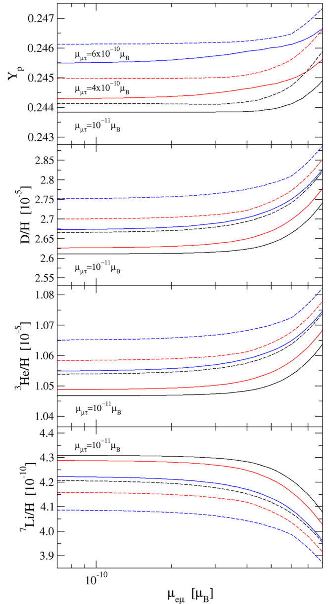
FIG. 6 (color online). The change in relative abundances of {}^4\text{He} , D , {}^3\text{He} , and {}^7\text{Li} as a function of the transition neutrino magnetic moment \mu_{e\mu} . The solid lines show the results when \mu_{e\tau} = 10^{-11} \mu_B (black— \mu_{\mu\tau} = 10^{-11} \mu_B , red— \mu_{\mu\tau} = 4 \times 10^{-10} \mu_B , and blue— \mu_{\mu\tau} = 6 \times 10^{-10} \mu_B ). The dashed lines are the results for \mu_{e\tau} = 6 \times 10^{-10} \mu_B with the colors representing the same values of \mu_{\mu\tau} that they did in the solid case.
