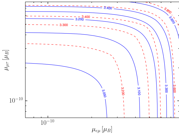
FIG. 9 (color online). Contours of constant N_{\text{eff}} in the \mu_{\mu\tau} versus \mu_{e\mu} plane. The solid contours correspond to \mu_{e\tau} = 10^{-10}\mu_B and the dashed contours correspond to \mu_{e\tau} = 4.9 \times 10^{-10}\mu_B .
