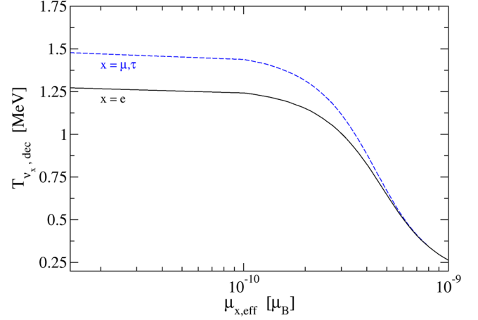
FIG. 4 (color online). Decoupling temperature of the three flavors as a function of their effective magnetic moment. The black solid line represents electron neutrinos which undergo weak decoupling at \sim 1.27 MeV. The blue dashed line represents muon and tau neutrinos which decouple weakly at \sim 1.48 MeV.
