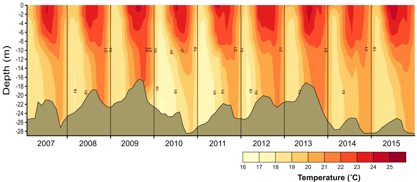
Figure 2 Vertical and temporal variation of temperature ( ^{\circ}\text{C} ) in Valle de Bravo reservoir from 2007 to 2015. Brown shade indicates the bottom below the reservoir.
