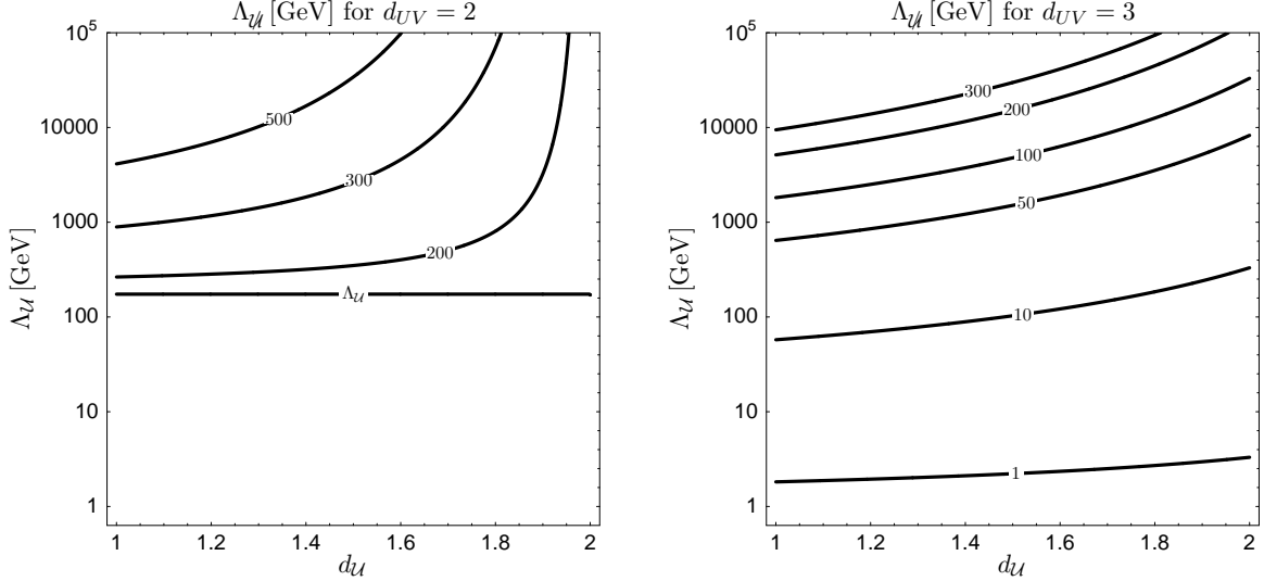
Figure 1: Contours of fixed CFT breaking scale, \Lambda_{\mathcal{U}} , as a function of the IR dimension of the unparticle operator, d_{\mathcal{U}} , and the scale at which it becomes conformal, \Lambda_{\mathcal{U}} . Two particular choices for the UV dimension of the unparticle operator are made, d_{UV} = 2, 3 .
