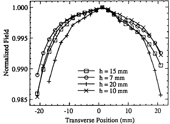
Figure 3. Transverse Profile of the Field for Different Half Gaps.
