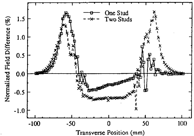
Figure 7. Transverse Scan Showing the Effect of Iron Inserts.
