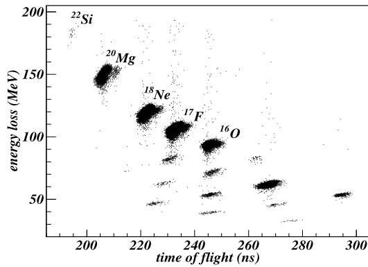
Fig. 1. Particle identification spectrum of energy loss from a large-area silicon detector versus time of flight between two plastic scintillators for secondary ions.
