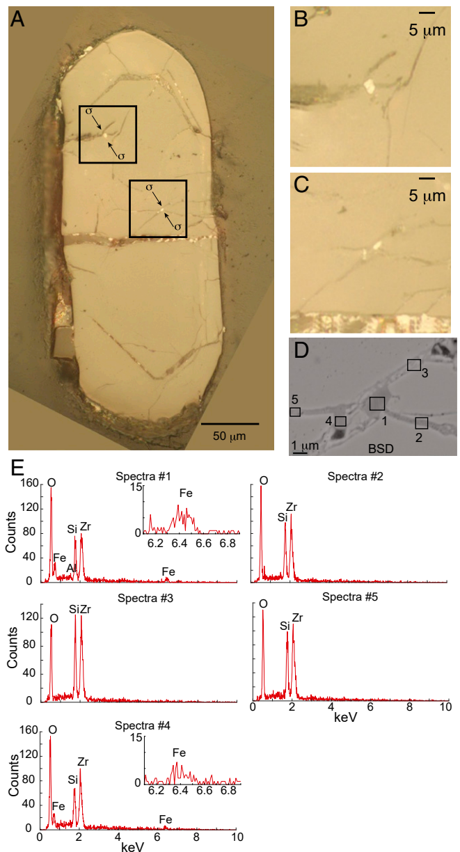
Fig. 3. Optical (reflected light) and SEM analyses of large (1 to 3 μm) magnetite inclusions in JH zircon. (A) Reflected light image (zircon RZ64). (B and C) Partially oxidized magnetite inclusions in crack. Other bright areas (at base) are other reflectors (i.e., not Fe). (D and E) SEM backscatter detector (BSD) image of region C with EDS analysis spots (1–5) and corresponding spectra (E). Also shown is possible stress orientation ( \sigma ) in A, suggesting cracks emanating from inclusion in B and C were formed under the influence of the same stress field.
