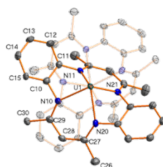
Figure 4. Structure of 2[OTf] 2 (left); Table compares the relevant bond distances of the three complexes. Further structural information can be found in the SI, Tables S1 and S2.
