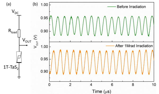
Fig. 3. (a) Circuit schematic diagram of a self-sustaining oscillator implemented with one 1T-TaS 2 device and a load resistor. (b) Oscillation waveform before and after 1 Mrad(SiO 2 ) X-ray irradiation.
