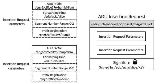
Figure 1. ADU Insertion Request and Insertion Request Parameters
