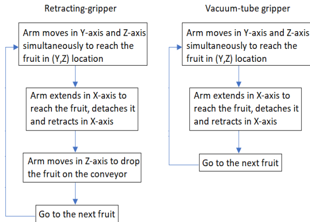
FIGURE 2. Harvest sequence for retracting-gripper and vacuum-tube gripper.
