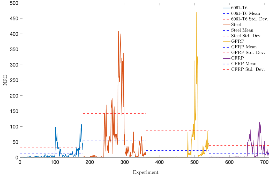
Figure 2.8: Normalized Residual Energy for the Plate Material perspective with the mean and standard deviation shown. From left to right are: 6061-T6, Steel, GFRP, and CFRP.
