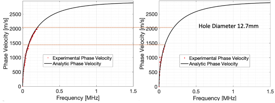
Figure 3.6: Side-by-side of 6061 Al w and w/o a 12.7mm hole with the analytic solution and WAVSVD approximation. The presence of a hole causes higher frequency phase velocity attenuation
