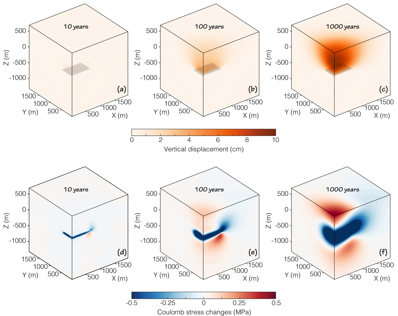
Fig. 11 Distribution of vertical displacement (a,b,c) and Coulomb stress changes (d,e,f) in a deep geological repository for the storage of nuclear waste 10, 100, and 1000 years after emplacement. Coulomb stress is
