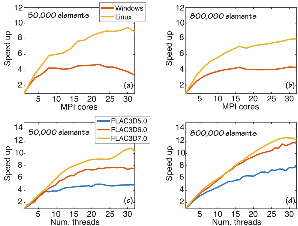
Fig. 1 Performance evaluation (speed up) for the individual codes on various hardware configurations. (a,b) TOUGH3 performance on two workstations operating on the same hardware configuration but running on different OS, for a computational mesh with 50,000 and 800,000 elements, respectively. (c,d) FLAC3D version 5, version 6, and version 7 performance on the Windows workstation, for a computational mesh with 50,000 and 800,000 elements, respectively
