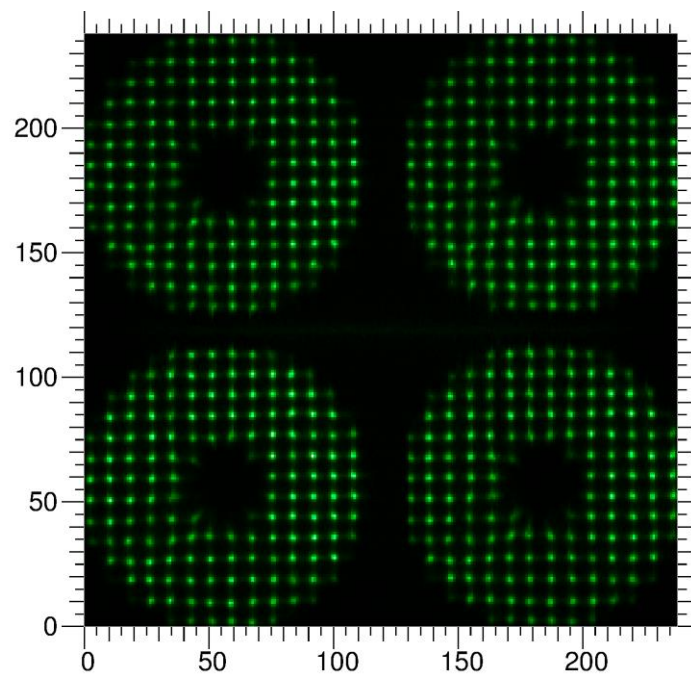
Figure 15: Shack-Hartmann patterns of the 4 Rayleigh LGS wavefront sensors imaged on the OCAM2-S camera using a temporal gate of 2 microseconds with a frame rate of 300Hz.
