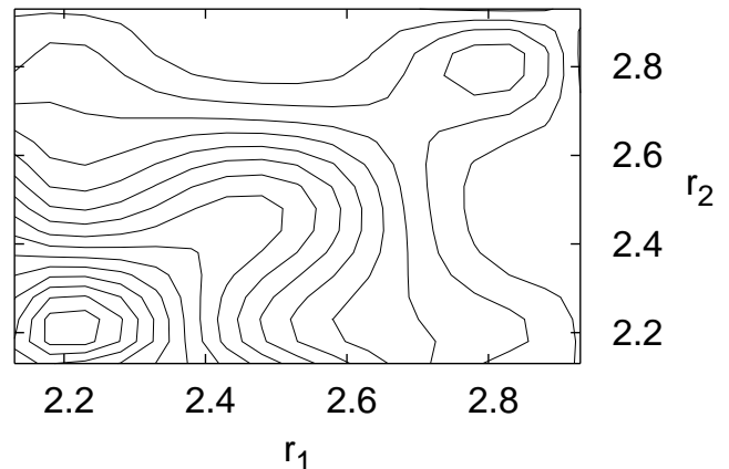
FIG. 6: Total width \Gamma of ^2B_1 state of H_2S^- at \theta_{HSH} = 92^\circ , contours every 4 \times 10^{-4} eV, where 1 \text{ eV} = 1.6021765 \times 10^{-19} \text{ J} .
