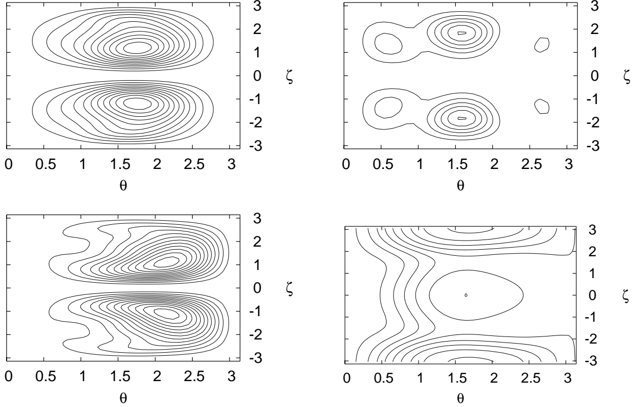
FIG. 7: Left to right, top to bottom: Modulus-squared of the entrance amplitude |V_{\bar{a}}|^2 for the \text{H}_2\text{S}^- \ ^2\text{B}_1 state at geometries (r_1, r_2, \theta_{HSH}) = (2.53, 2.53, 92^\circ) , (2.13, 2.93, 92^\circ) , and (2.53, 2.13, 92^\circ) , internormalized. Bond lengths, units of a_0 . Bottom right, phase of entrance amplitude V_{\bar{a}} at (2.53, 2.53, 92^\circ) , contours every 0.157 radians.
