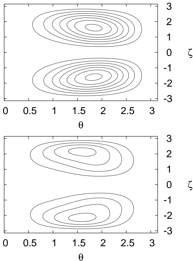
FIG. 3: Modulus-squared of the entrance amplitude |V_{\bar{a}}|^2 for the \text{H}_2\text{O}^- \ ^2\text{B}_1 state at geometries (r_1, r_2, \theta) = (1.81, 1.81, 104.5^\circ) and (1.81, 2.11, 104.5^\circ) , internalized, bond lengths, units of a_0 , where 1 a_0 = 5.2917721 \times 10^{-11} m.
