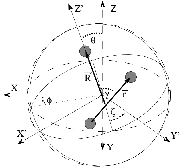
FIG. 11: ‘‘R-embedding’’ coordinate system used in this calculation. The origin is the center of mass. The body-fixed (BF) frame is labeled by the X' , Y' , and Z' axes; the space-fixed (SF), by X , Y , and Z . The BF axes are marked with thin lines, and the BF X'Z' and X'Y' planes are both marked with a thin line circle. The SF axes are marked with dashed lines, and the SF XZ and XY planes are marked with dashed circles. The molecule resides in the BF X'Z' plane. The Euler angles \phi , \theta , and \zeta orient the BF frame with respect to the SF frame. The line of nodes is also drawn. The \vec{r} vector connects the nuclei of the diatomic. The \vec{R} vector connects the center of mass of the diatomic to the third atom and is collinear with the BF Z' axis. R is the length of \vec{R} , r is the length of \vec{r} , and \gamma is the angle between the \vec{R} and \vec{r} vectors.
