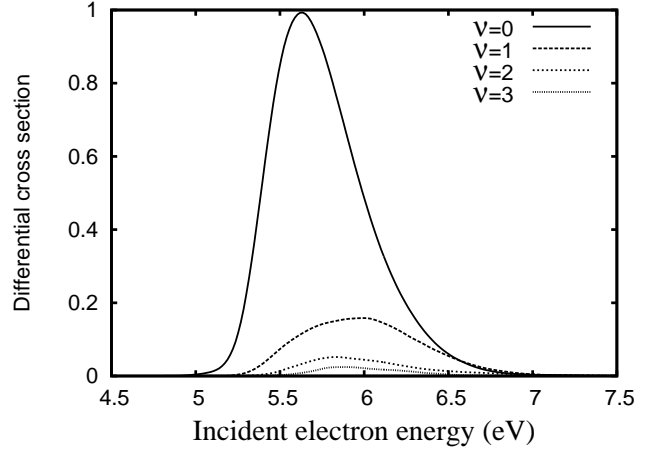
FIG. 12: Differential cross section for \text{H}^- + \text{SH}(\nu) from \text{H}_2\text{S} at scattering angle \theta = 45^\circ , arbitrary units.
