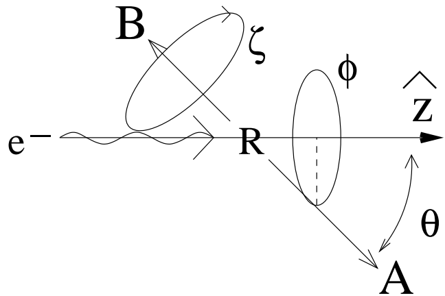
FIG. 2: Schematic of Euler angles \phi, \theta, \zeta and dissociative coordinate R for general dissociative attachment problem. ‘‘A’’ and ‘‘B’’ stand for one or more atomic fragments of molecule AB and R is the distance between their centers of mass. A is the anion.
