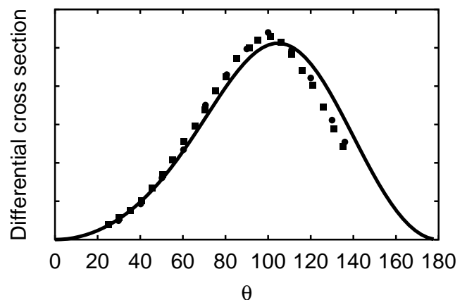
FIG. 5: Angular distribution of \text{H}^- from \text{H}^- + \text{OH} via dissociative attachment to the ^2\text{B}_1 state, assuming axial recoil, along with the measurements of Belič, Landau, and Hall [10] (squares) and Trajmar and Hall [9] (circles), arbitrary units.
