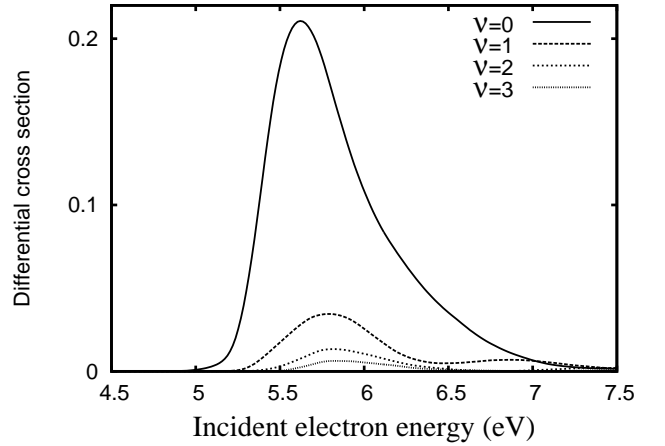
FIG. 13: Differential cross section for \text{H}^- + \text{SH}(\nu) from \text{H}_2\text{S} at scattering angle \theta = 165^\circ , arbitrary units.
