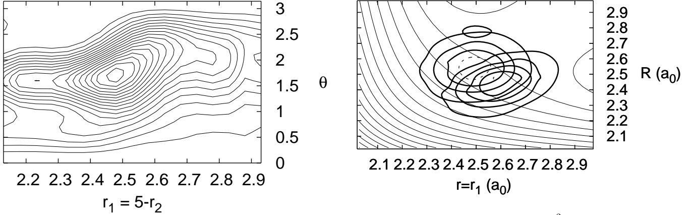
FIG. 9: Square of driving term |\phi_{\nu_i}|^2 for initial wavepacket, normalized to unity, \Lambda = 1 calculation, integrated over Jacobi angle \gamma , for \theta = 45^\circ (circular) and 165^\circ (oblong) calculations, with potential energy surface at \gamma = 92^\circ , contours every 0.25eV. Distances in units of a_0 .
