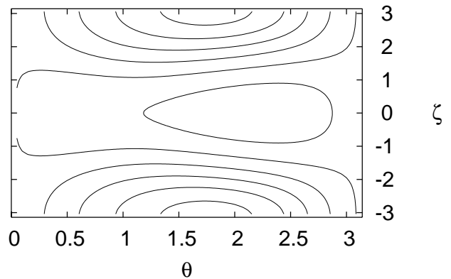
FIG. 4: Phase of the entrance amplitude V_{\bar{a}} for the \text{H}_2\text{O} \ ^2\text{B}_1 state, at geometry (r_1, r_2, \theta_{HOH}) = (1.81, 1.81, 104.5^\circ) , contours every 0.157 radians. Bond lengths, units of a_0 .
