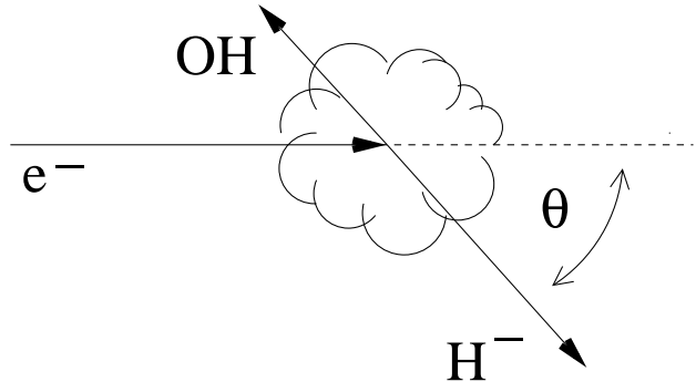
FIG. 1: Definition of H^- scattering angle \theta .
