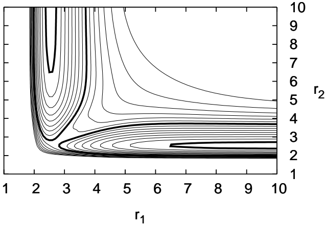
FIG. 10: Fitted H 2 S potential surface at \theta_{HSH} = 92^\circ , with contours every 0.25eV. Bond lengths in units of a_0 .
