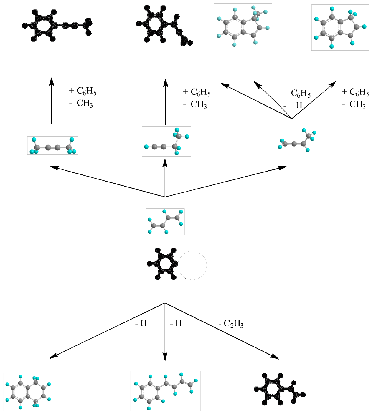
Figure 6: Summary of primary (bottom) and secondary reaction products (upper section) probed in the present experiment.
