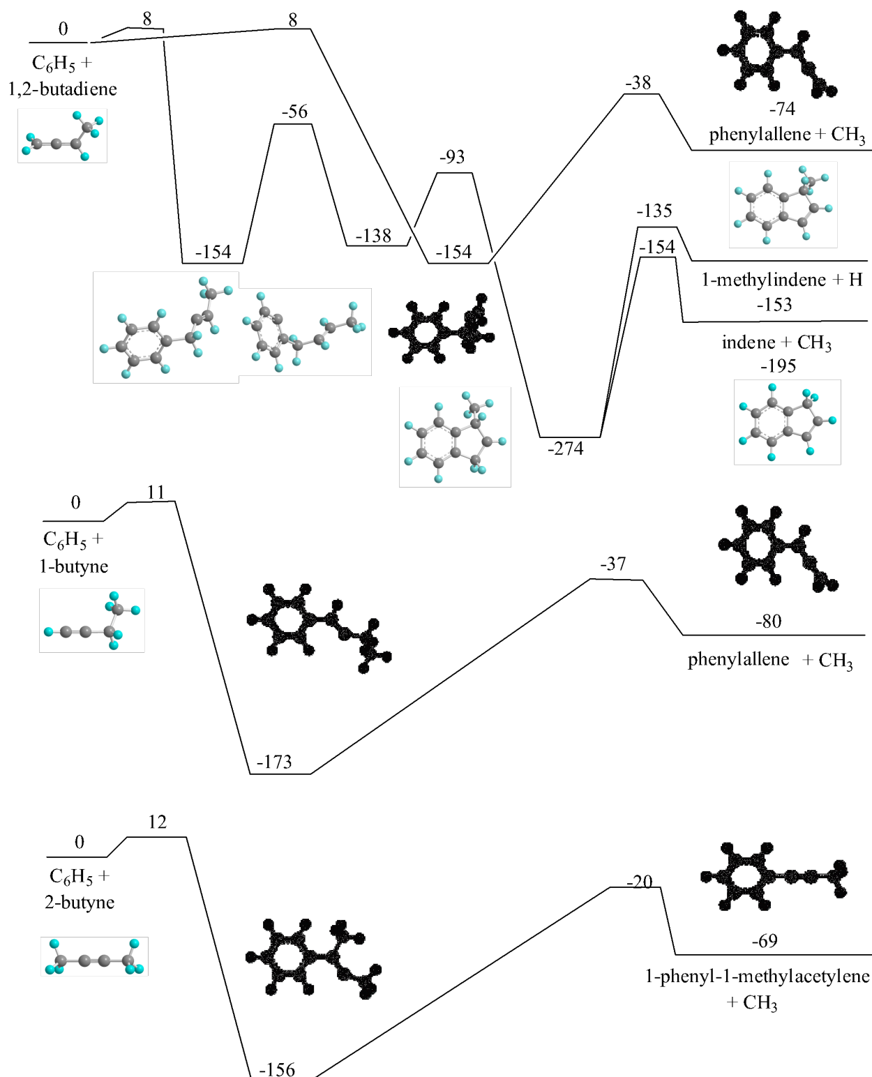
Figure 5: Formation of secondary reaction products via the reactions of phenyl radicals with 1,2-butadiene, 1-butyne, and 2-butyne. Relative energies in kJ mol -1 are computed at the G3(MP2,CC)//B3LYP/6-311G** level of theory.
