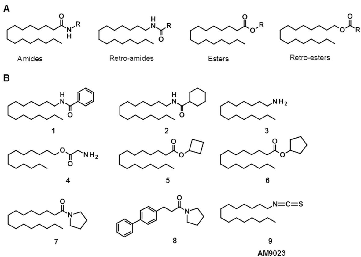
Fig. 2. (A) Chemical structures of amides, retro-amides, esters, and retro-esters of palmitic acid. (B) Chemical structures of selected NAAA inhibitors.
