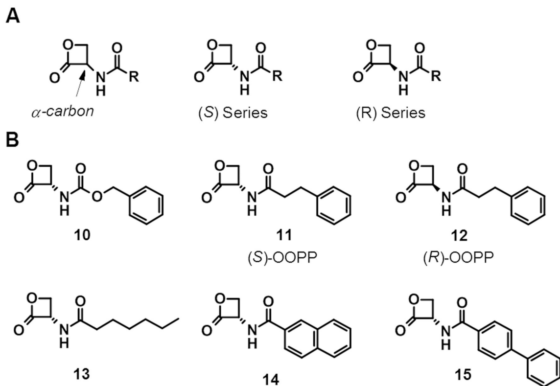
Fig. 3. (A) General structures of serine-derived \beta -lactones. (B) Chemical structures of selected serine-derived \beta -lactone NAAA inhibitors.
