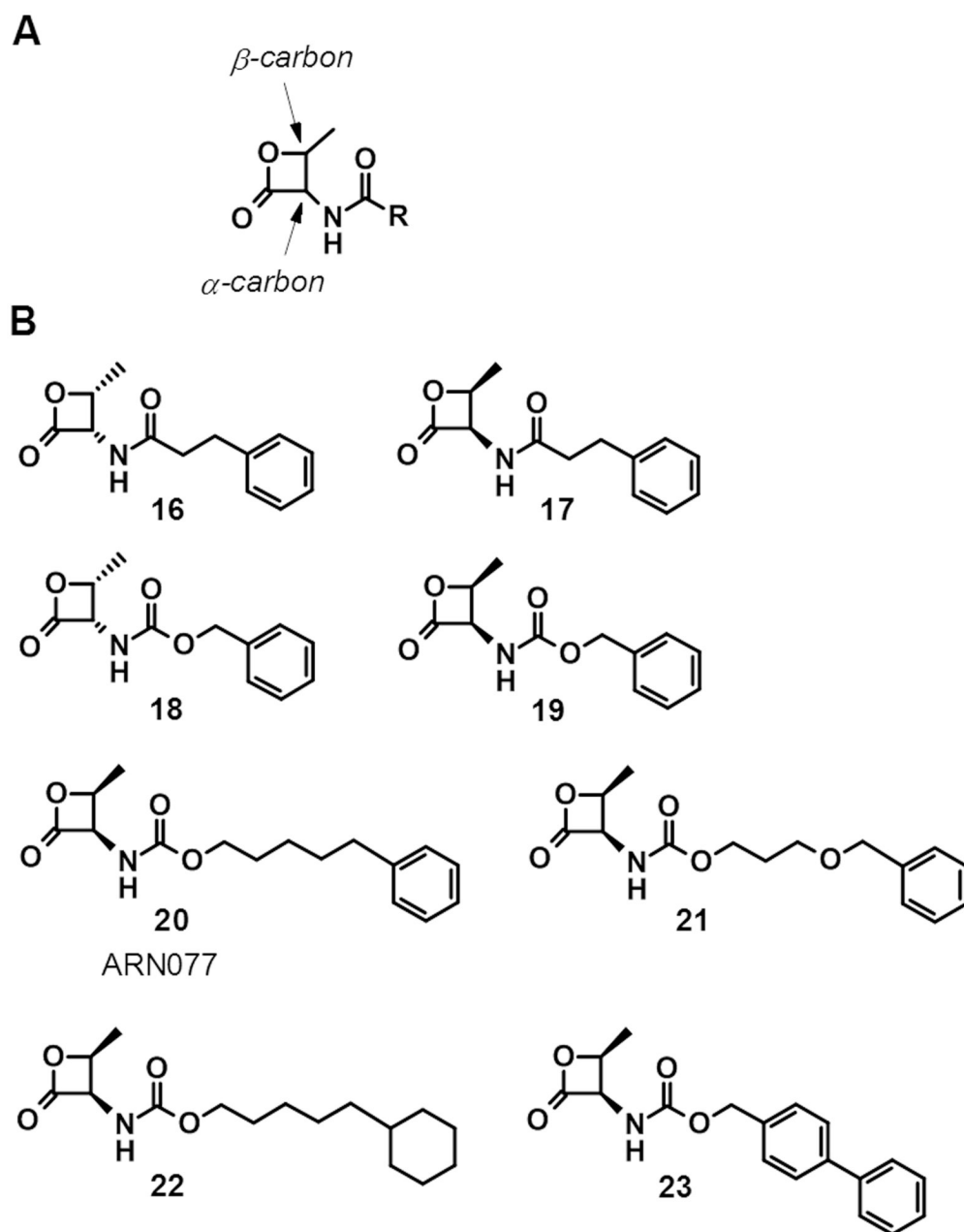
Fig. 4. (A) General structure of threonine-derived \beta -lactones. (B) Chemical structures of selected threonine-derived \beta -lactones.
