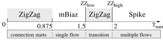
Fig. 10. ZBS scheme (when bottleneck link is not underutilized). Axis T_{narr} = T_{avg}/T_{min} , where T_{avg} is the average packet interarrival time and T_{min} is the minimum packet interarrival time.
