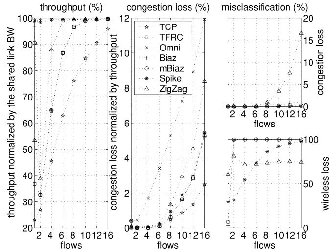
Fig. 9. Competition in the WB topology.
