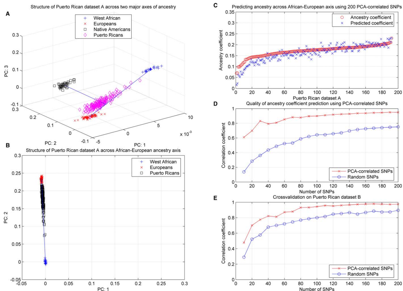
Figure 6. Applying PCA-Correlated SNPs for Structure and Ancestry Prediction of the Admixed Puerto-Rican Population
