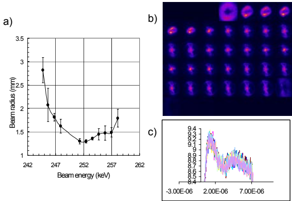
FIG.12. shows (a) variation of neutralized beam radius corresponds to beam energies (b) beam pattern from head to tail by varying time delay of image recording, (c) variation of multiple Marx waveforms for a same condition.
