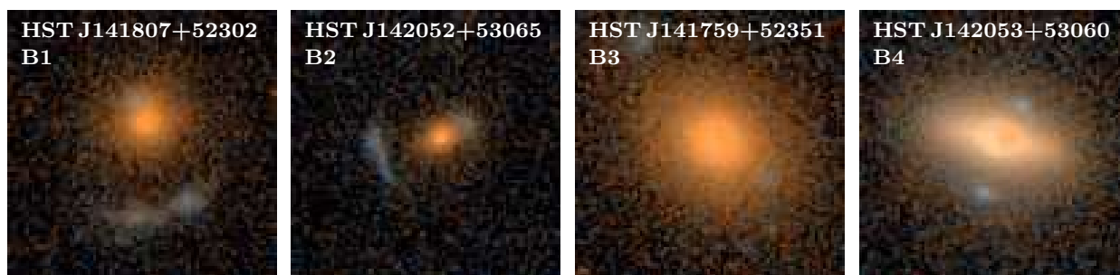
Fig. 2.— Additional lens candidates based on visual inspection, but not yet bolstered by spectroscopy. The left two are candidate arc/counter-arc lenses, whereas the right two are candidate two-image lenses. Images are 3 arcsec square.
