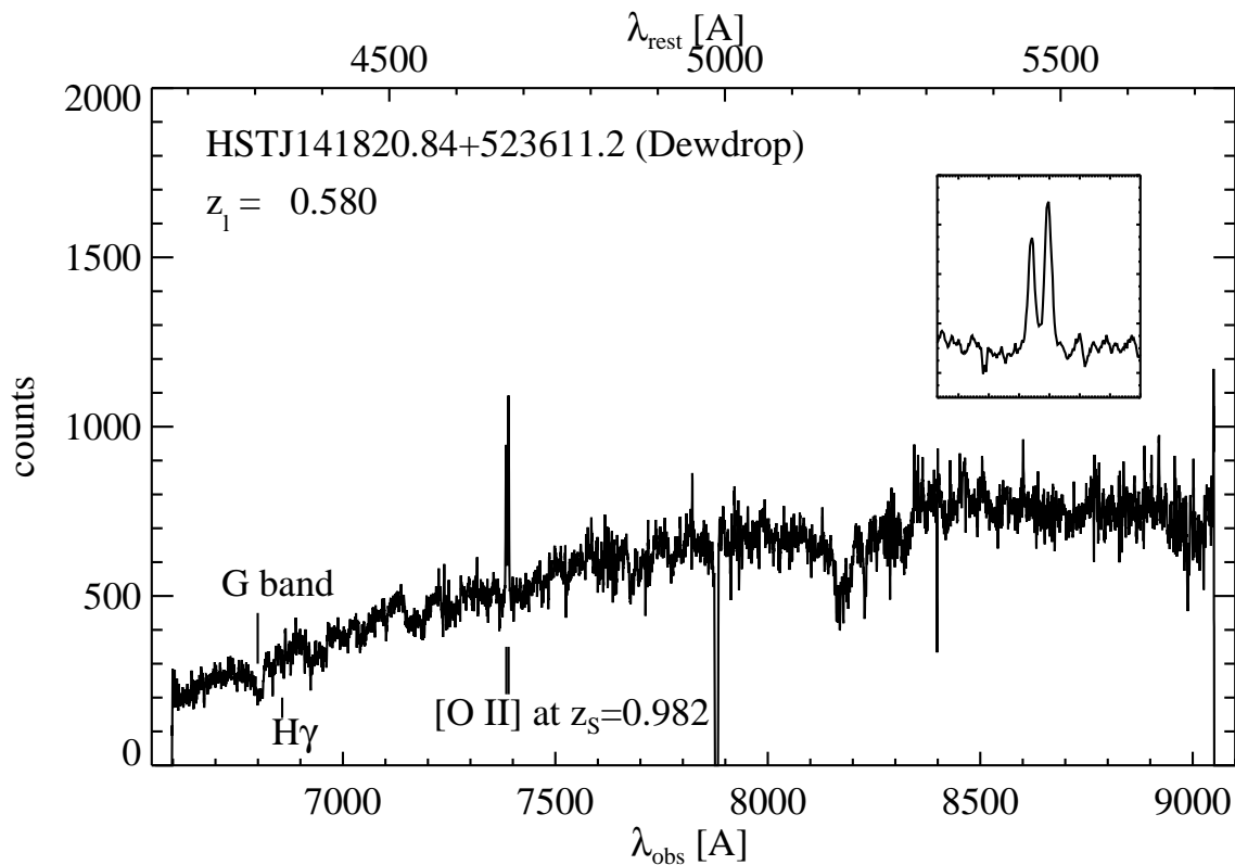
Fig. 3.— The DEIMOS spectrum of the Dewdrop lens clearly shows an “anomalous” doublet emission line (insert), which is readily identified as [\text{O II}] at z_{\text{source}} = 0.9818 .
