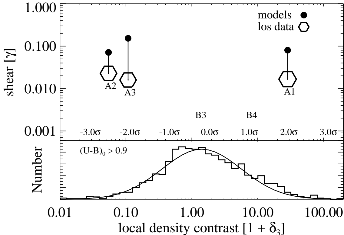
Fig. 4.— The distribution of the local-environmental measure 1 + \delta_3 (Cooper et al. 2005a), for “red sequence” galaxies with rest-frame colors (U - B)_0 > 0.9 (valid for all lenses here), including N\sigma deviations from the mean. Upper panel: The shear for each lens, inferred through the lens models (filled-circles), and through the simple SIS-based line-of-sight influence (open hexagons). The 1 + \delta_3 values of the lens-candidates B3 and B4 are shown as well.
