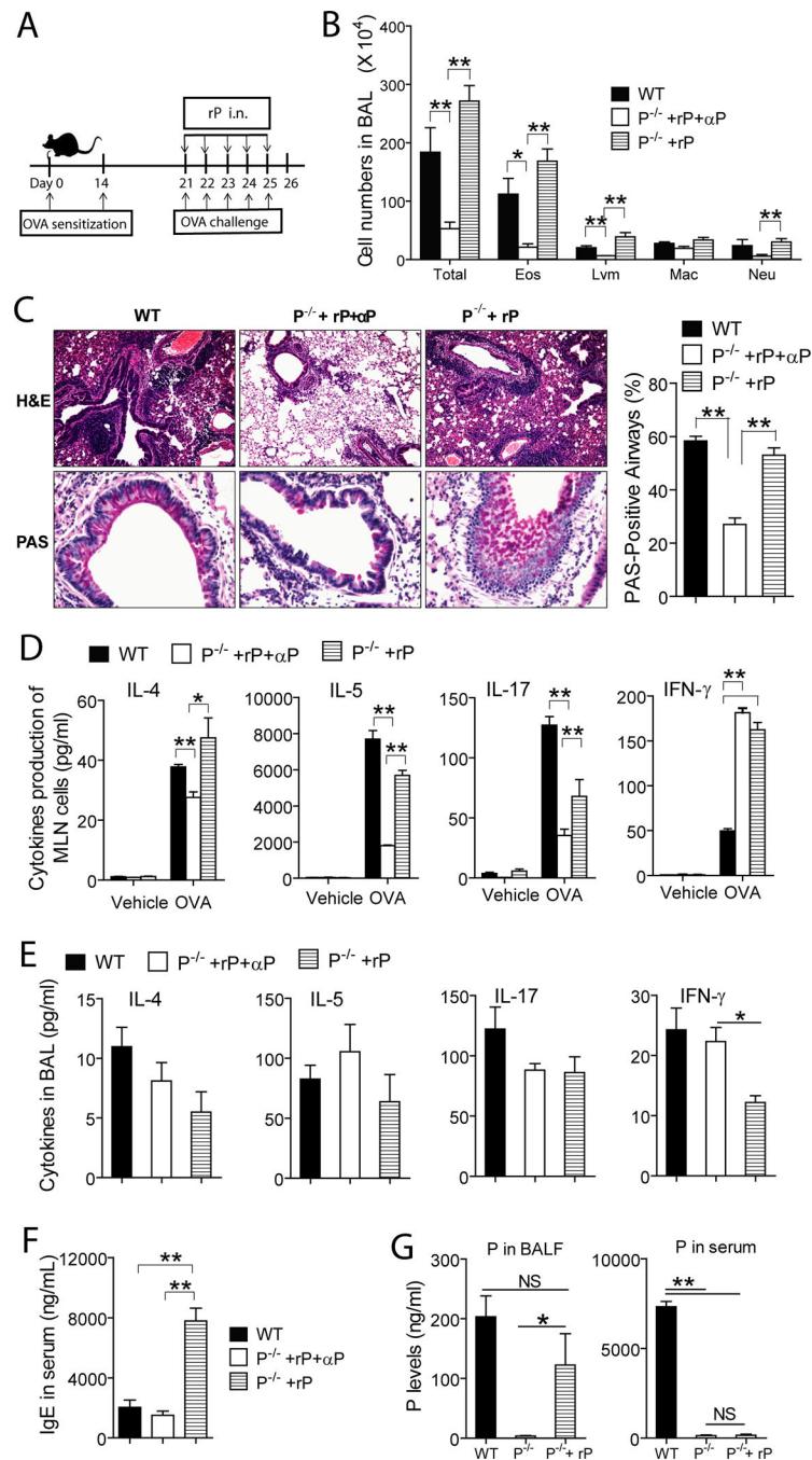
Fig. 7. Local reconstitution of properdin in the airways of P^{-/-} mice restores their sensitivity to OVA-induced asthmatic lung inflammation and increases Th2 and Th17 immune responses (A) P^{-/-} mice were treated intranasally with recombinant P or recombinant P plus anti-P mAb ( \alpha P) prior to each OVA challenge as indicated. (B) Differential cell counts in BAL showing that P^{-/-} mice reconstituted with recombinant P had much higher numbers of total inflammatory cells, eosinophils (Eos), lymphocytes (Lym) and neutrophils (Neu) than P^{-/-} mice reconstituted with recombinant P plus anti-P mAb. The number of total cells, eosinophils and lymphocytes in P reconstituted P^{-/-} mouse BAL were even higher than those of WT mice. Mac, macrophages. (C) Representative H&E and PAS staining showing
