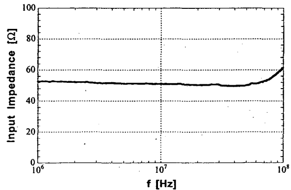
Fig. 2. Magnitude of the impedance seen at the input of the charge sensitive loop of figure 1 as a function of frequency.
