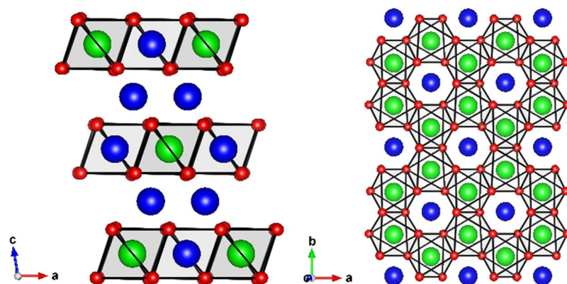
Figure 1. Left: \text{Li}_2\text{MO}_3 ( M = 4d or 5d element) structure as alternating \text{LiM}_2 and \text{LiM} layers. Right: Viewed along the c axis the \text{LiM}_2 layer, where \text{MO}_6 edge-sharing octahedra form the honeycomb lattice. Blue, green, and red spheres represent lithium, metal, and oxygen atoms respectively.
