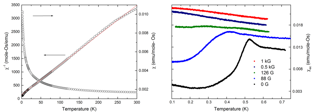
Figure 6. Left: DC-Susceptibility \text{Li}_{2.15}\text{Os}_{0.85}\text{O}_3 versus temperature. Also shown is the inverse susceptibility after subtracting a van Vleck term as described in the text. Right: ac-susceptibility versus temperature at different values of applied magnetic field. The curves have been offset vertically by 0.0020, 0.0032, 0.0044, and 0.0056 emu for H = 88, 126, 500 , and 1000 G respectively, for clarity.
