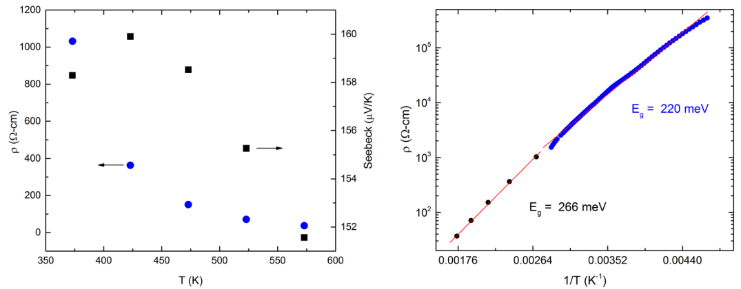
Figure 5. Left: High temperature resistivity and Seebeck coefficient data of \text{Li}_{2.15}\text{Os}_{0.85}\text{O}_3 sample from 350 to 600 K. Right: Resistivity versus temperature for \text{Li}_{2.15}\text{Os}_{0.85}\text{O}_3 in the range 200–600 K versus inverse temperature. The low and high temperature measurements were performed in different apparatuses on samples from the same growth run. To assure continuity at T = 300 K, the data have been rescaled for the low temperature measurement due to its greater uncertainty in the geometric factor.
