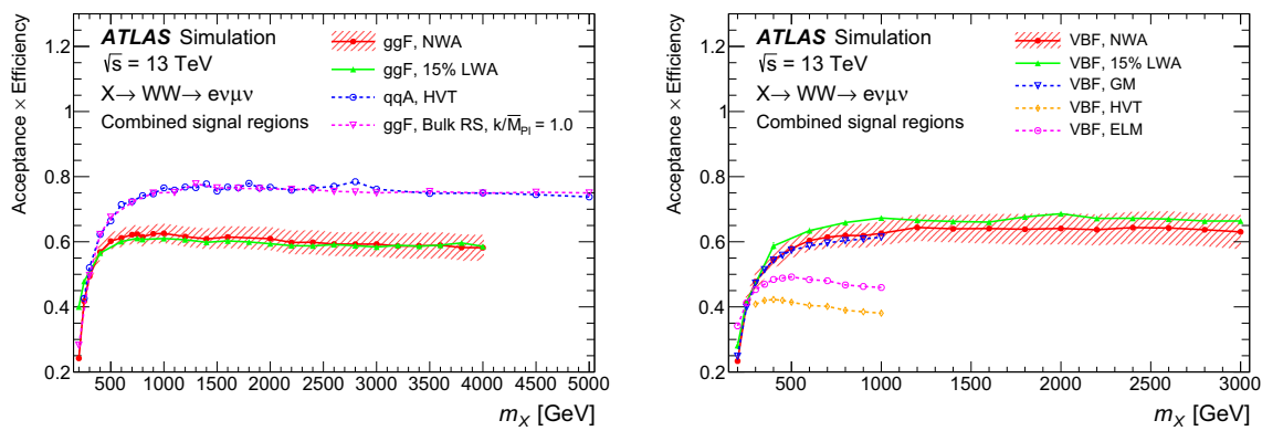
Fig. 1 Acceptance times efficiency as a function of signal mass for the ggF or qqA (left) and VBF (right) productions. All three signal event categories are combined. The hatched band around the NWA signal curve shows the typical size of the total statistical and systematic uncertainties
