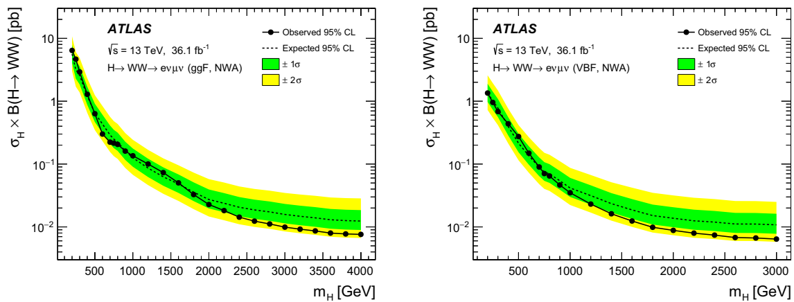
Fig. 5 Upper limits at 95% CL on the Higgs boson production cross section times branching fraction \sigma_H \times B(H \rightarrow WW) in the ev\mu\nu channel, for ggF (left) and VBF (right) signals with narrow-width lineshape
