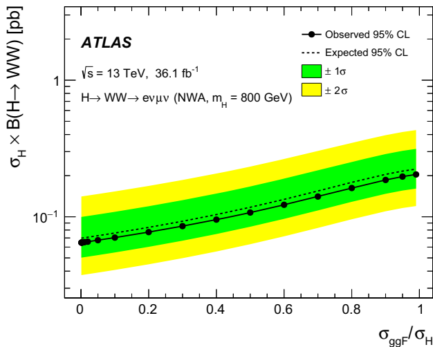
Fig. 6 Upper limits at 95% CL on the total ggF and VBF Higgs boson production cross section times branching fraction \sigma_H \times B(H \rightarrow WW) in the ev\mu\nu channel, for a signal at 800 GeV as a function of the ggF cross section divided by the combined ggF and VBF production cross section. The inner and outer bands show the \pm 1\sigma and \pm 2\sigma ranges around the expected limit
