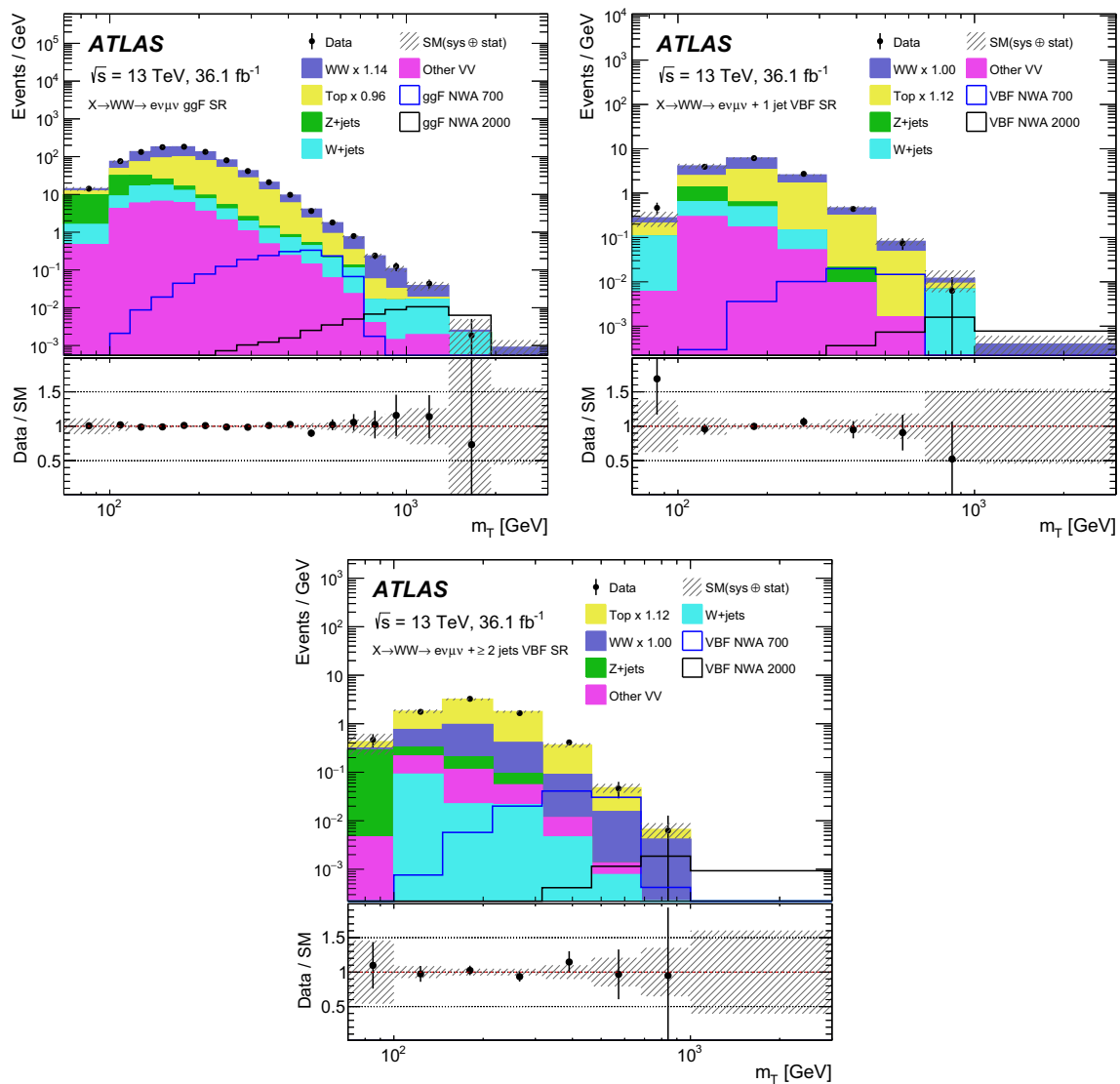
Fig. 4 Post-fit distributions of the transverse mass m_T in the SR_{ggF} (top left), SR_{VBF1J} (top right) and SR_{VBF2J} (bottom) categories. In each plot, the last bin contains the overflow. The hatched band in the upper and lower panels shows the total uncertainty of the fit. The top-quark and WW background event yields are scaled using the indicated nor-
