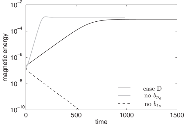
FIG. 5. Times series of the magnetic energy in the cases where either the coefficients b_{pe} or the coefficients b_{to} of the m = 1 magnetic field are suppressed, compared with that for the full MHD simulation in Case D. All the cases have similar wall parameters. A global magnetic diffusion time is \tau_\eta = \text{Rm} = 300 .
