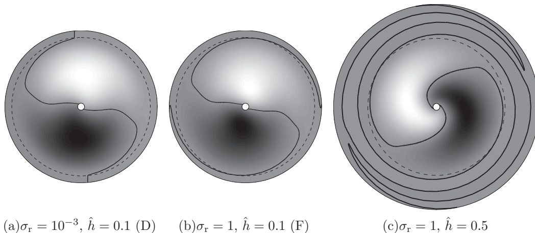
FIG. 8. Radial magnetic field B_r in a conical section (r, \phi) at colatitude \theta = \pi/6 . The dashed line indicates the fluid-wall interface, and the solid bold line is the contour B_r = 0 (not a magnetic field line).
