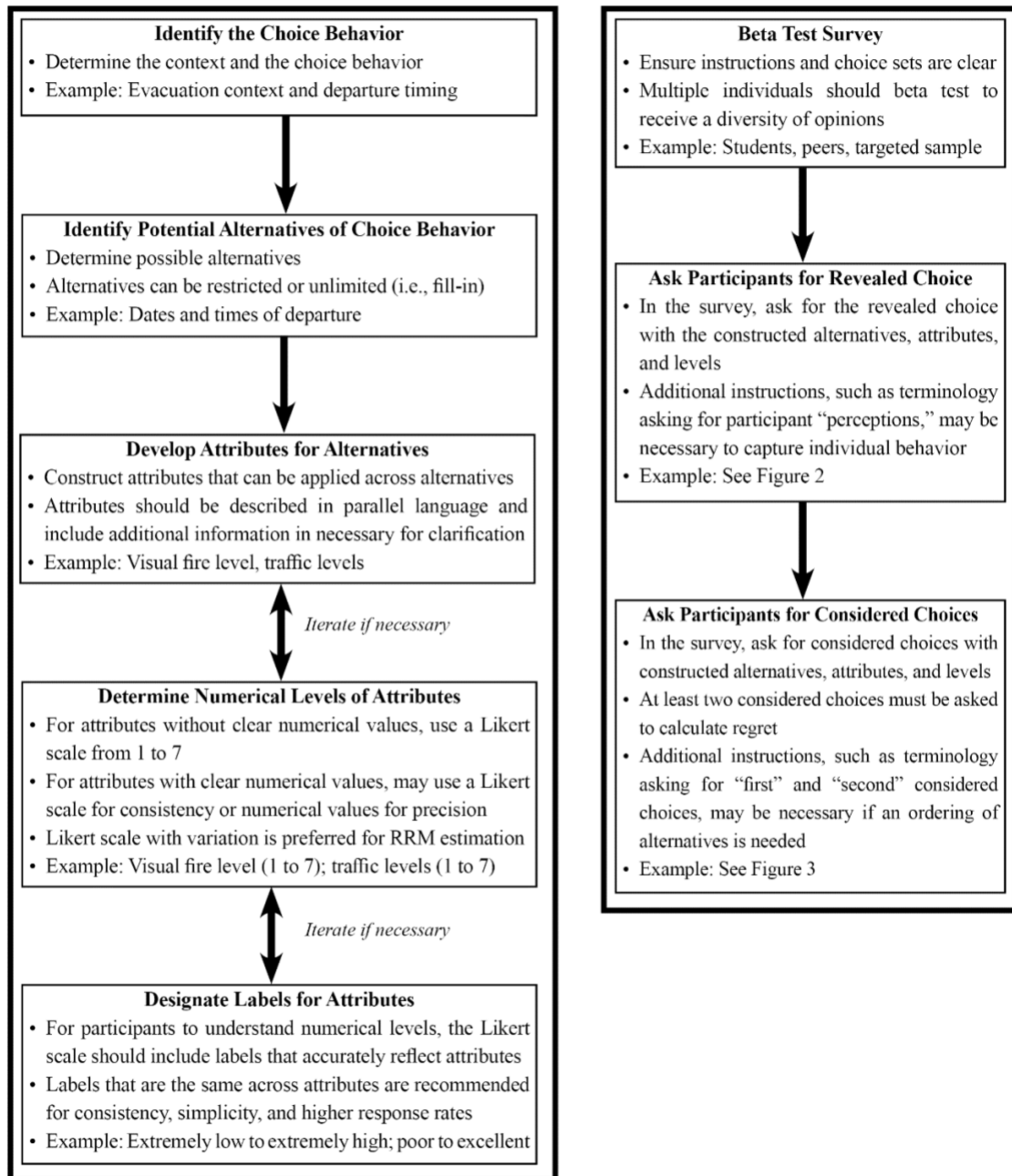
Figure 1 RP Survey Methodology for RUM and RRM Models
