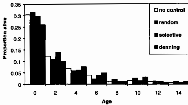
Figure 1. Computer model projections of the proportion of coyotes alive after 10 years of exposure to various control techniques: no control, selective removal of alpha males and females, and removal of litters of puppies.
