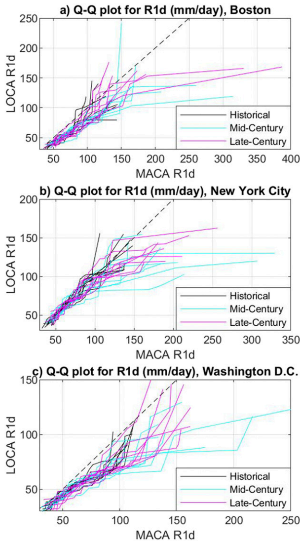
FIG. 9. The eight-model ensemble of Q–Q plot for the annual maximum 1-day precipitation (R1d; mm day -1 ) between LOCA and MACA in historical, midcentury, and late-century climates, for three metropolitan areas: (a) Boston, (b) New York City, and (c) Washington, D.C. Each solid line represents one model, and the 1:1 line is dashed.
