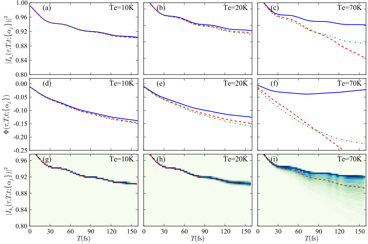
Figure 2: Traces (a-c) and distribution (g-i) of the non-integrated three-pulse photon echo |I_{k_s}(\tau, T, t; \{\alpha_j\}_i)|^2 of a single molecule at t = \tau = 10\text{fs} for different temperature T_e = 10\text{K} , 20\text{K} and 70\text{K} . The corresponding dynamics of the phase factors \Phi(\tau, T, t; \{\alpha_\xi\}_i) are presented in (d-f). In the simulation, the other parameters are \omega_c = 53\text{cm}^{-1} and \lambda = 100\text{cm}^{-1} . In the each trace, we use the same initial environmental state \{\alpha_\xi\}_i in Eq.(5) at each calculated time point and evaluate the signal as a function of population time T . For different traces, we randomly choose the initial states \{\alpha_\xi\}_i , where i is the index of the trace. For a specific mode ( \omega_\xi ), its initial states (the set of \alpha_\xi^{(i)} ) in the different traces are randomly generated using the GSL bivariate Gaussian distribution random number generator 25 according to the Gaussian distribution in Eq. (6). Three typical traces are shown to demonstrate the effect of differing initial states. The decay behaviors of these traces follow the corresponding dynamics of the phase factors \Phi(\tau, T, t; \{\alpha_\xi\}_i) in (d-f). In (g-i), we illustrate the distribution of signal intensity, estimated from 5000 traces. The color indicates the relative probability of the signal strength at certain time. The red dotted line represents the signal averaged over these traces.
