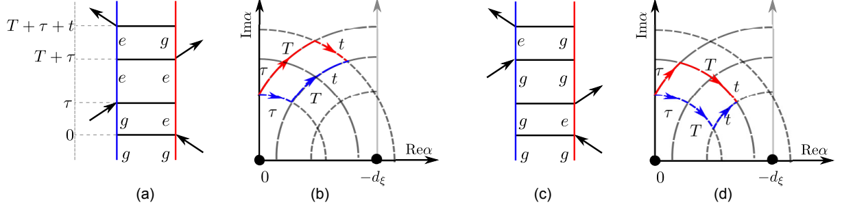
Figure 1: Double side Feynman diagrams of the response functions R_1(\tau, T, t; \{\alpha_\xi\}) and R_2(\tau, T, t; \{\alpha_\xi\}) and the corresponding phase-space traces of environmental DoF. To explicitly illustrate the evolution, we adapt one particular environmental DoF. (a) Diagram of electronic DoF in the excited state population pathway. The first pulse creates a coherence that evolves for time \tau , then the second pulse creates an excited-state population that evolves for time T . The third pulse creates a coherence that cancels the phase accumulated during time \tau . (b) The corresponding evolution of the vibrational state in phase-space of pathway in (a). As demonstrated in Supporting Information, the coherent state can be characterized with a complex number. In (b), we denote a coherent state as a point in the complex plane. The evolution of coherent state leaves a trace in this complex plane. During the coherent time [0, \tau] , the ket and bra evolve under different Hamiltonians H_e and H_g , which correspond to the red and blue arcs on circles centered at z = 0 and z = -d_\xi in complex plane. The two states move far away from each other. During the population time [\tau, T + t] , the ket and bra follow the same Hamiltonian H_e . However, the radii of the circles are different, as illustrated in (b). Therefore, they separate further. In the second coherence time [\tau + T, \tau + T + t] , the distance between two states decreases in the complex plane. These processes are equivalent to the rephasing of electronic DoF in (a). (c) Shows the electronic DoF propagating in the ground state population path-way during the population period. (d) The corresponding evolution of the environmental DoF in the phase space.
