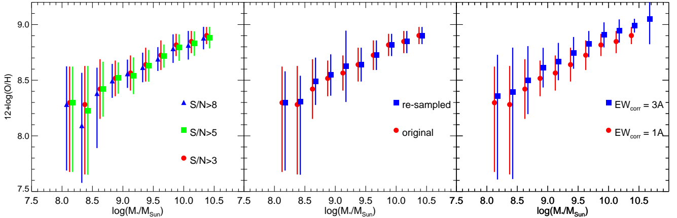
FIG. 9.— Selection and measurement effects on our MZR measurement. In all panels, red circles with error bars are the median and 16th and 84th percentiles of the DEEP3+TKRS “upper+lower Z” MZR with S/N_{[\text{OIII}] \text{ and } H\beta} > 3 and H\beta EW correction of 1 \text{ \AA} (the same as that in Panel (a) of Figure 5). Left: S/N cut effect. Blue triangles and green squares show the re-calculated MZRs with S/N_{[\text{OIII}] \text{ and } H\beta} > 8 and 5 , respectively. Middle: Sample bias effect. Blue squares and error bars show the MZR of re-sampling our DEEP3+TKRS sample to match the SSFR distribution at a given M_* of our parent samples. This panel tests the effect of our final sample being biased toward slightly high-SSFR galaxies (see Figure 1). Right: H\beta EW correction effect. Blue squares and error bars show the MZR calculated with H\beta EW correction factor of 3 \text{ \AA} .
