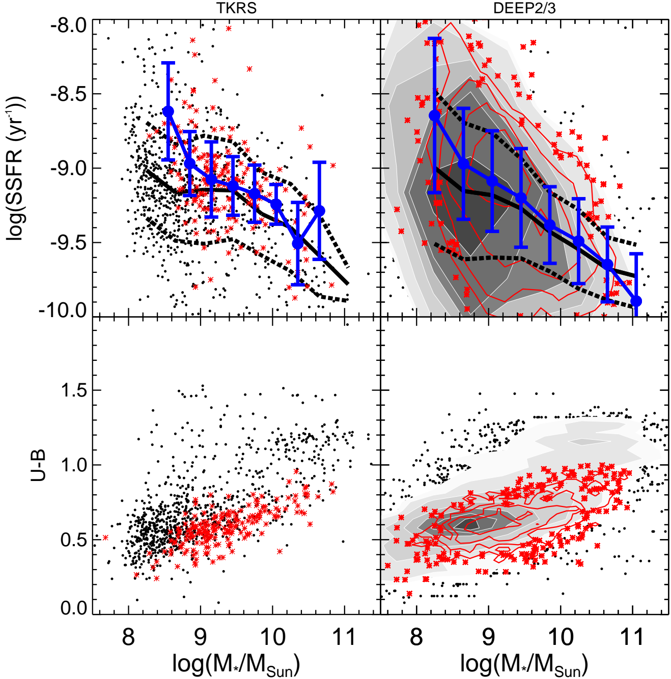
FIG. 1.— Sample properties. The SSFR- M_* and U-B color- M_* relations of the galaxies in our sample are plotted as red symbols (plus red contours for DEEP2/3). For each survey (as shown by the title of the upper panels), the mean and 1\sigma scatter of the SSFR- M_* relation of our sample are shown by large blue circles with error bars. Over-plotted black dots (plus gray contours for DEEP2/3) are the mass-complete parent samples, constructed with galaxies with 0.5 \leq z \leq 0.7 and H < 25.0 from CANDELS/GOODS-N (left column) catalog and m_{3.6\mu\text{m}} < 24 from EGS (right column). The mean and 1\sigma scatter of star-forming galaxies (SSFR > 10^{-10} /yr) in the parent samples, i.e., the star-forming main sequence at 0.5 \leq z \leq 0.7 , are shown by solid and dashed black lines.
