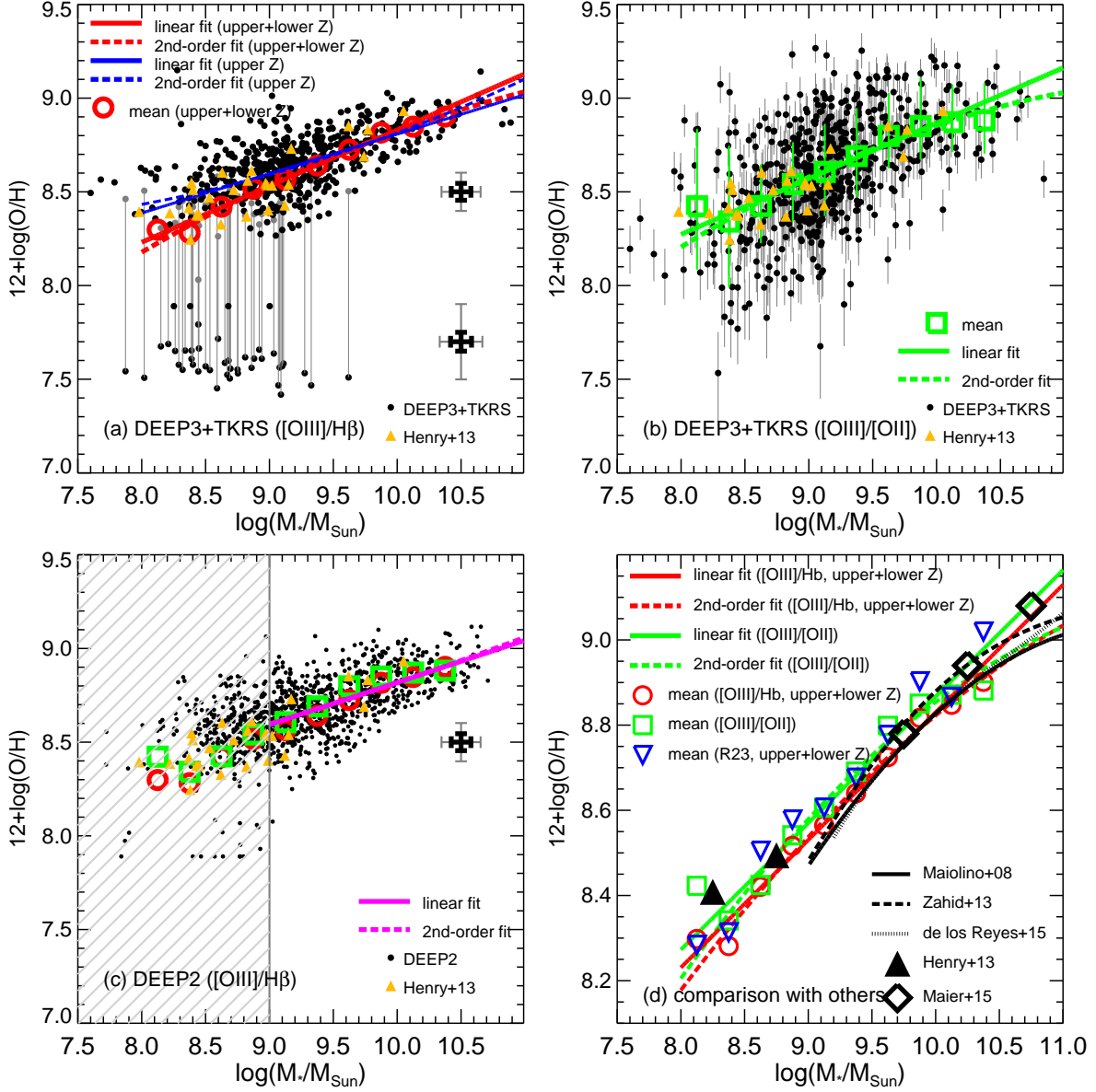
FIG. 5.— (a): MZR of our DEEP3+TKRS sample with metallicity measured through [\text{OIII}]/\text{H}\beta . Black circles are the metallicity of each galaxy after breaking the lower–upper branch degeneracy using the threshold in Figure 4. For each lower-branch galaxy, we also show its upper-branch metallicity with a gray vertical line. The means, best linear fit, and best second-order polynomial fit of the metallicity after breaking the degeneracy (“upper+lower Z”) are shown by red open circles, solid line, and dashed line. As a reference, the blue solid and dashed lines show the best linear and second-order polynomial fits of the sample using the upper-branch metallicities (“upper Z”) for all galaxies. The upper and lower black (gray) error bars show the median (90 percentile) measurement uncertainty of the upper and lower branches, respectively. (b): MZR of our DEEP3+TKRS sample with metallicity measured through [\text{OIII}]/[\text{OII}] . The means, best linear fit, best second-order polynomial fit are shown by green open squares, solid line, and dashed line. (c): MZR of our DEEP2 sample with metallicity measured through [\text{OIII}]/\text{H}\beta . All galaxies use their “upper Z”. Galaxies at M_* < 10^9 M_\odot (shaded area) are significantly subjected to the branch degeneracy and hence not used in our analyses. The best linear and second-order polynomial fits are shown by purple solid and dashed lines. The means of DEEP3+TKRS are shown as open circles ( [\text{OIII}]/\text{H}\beta -derived “upper+lower Z”) and squares ( [\text{OIII}]/[\text{OII}] -derived). Data from H13, after being converted to the M08 metallicity calibration, are shown as yellow triangles in Panel (a), (b), and (c). (d): Comparison between our MZRs and other measurements in the literature. Red and green lines and symbols are the same as in Panel (a), (b), and (c). We also add the mean metallicity measured through R23 in this panel (blue triangles). Black curves and symbols show the MZRs at similar redshifts from other studies, as the labels indicate. The y-axis range of Panel (d) is different from that of other panels.
