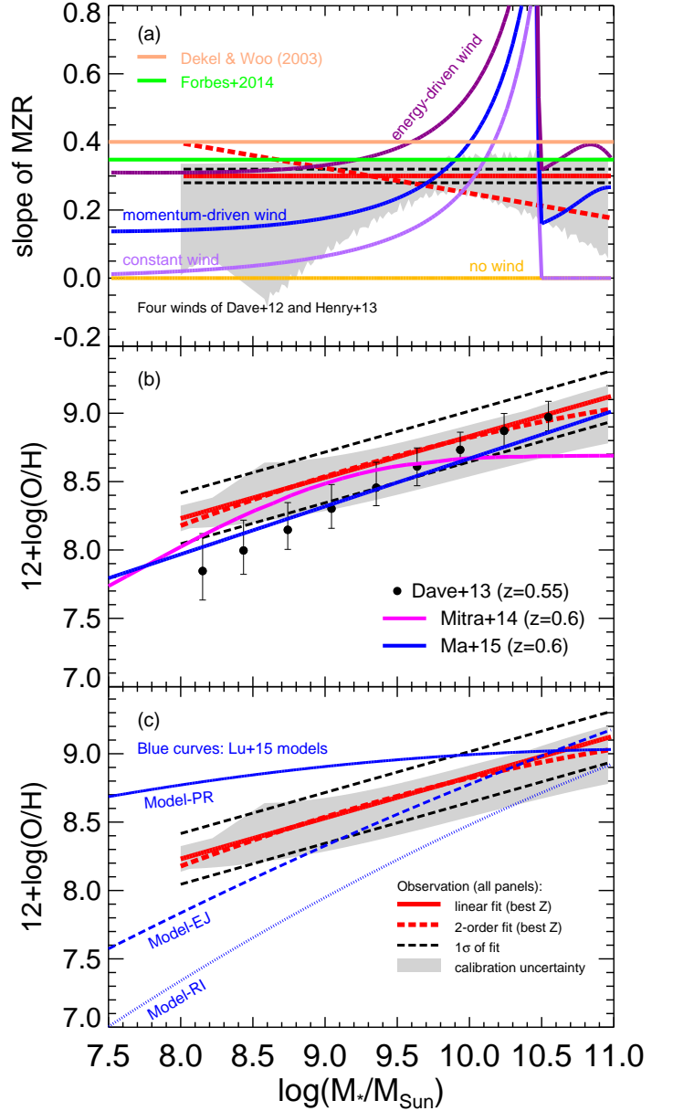
FIG. 8.— Comparisons between our MZR and others from theoretical works. In all panel, red solid and dashed lines are best-fit linear and second-order polynomial functions of the DEEP3+TKRS sample, galaxies in which break their lower-upper branch degeneracy by using [\text{OIII}]/[\text{OII}] (“upper+lower Z”). The black dashed lines are the 1\sigma range of the best linear fit. The gray shaded area is the calibration uncertainties of different metallicity calibrations (Sec. 6.1). Top (a): Slope of the MZRs. Slopes from theoretical works, as the text shows, are over-plotted against our slopes. The sharp discontinuity of wind models around M_* = 10^{10.5}M_\odot is due to the fact that \alpha_Z term in Equation 4 becomes abruptly independent on M_{\text{halo}} at M_{\text{halo}} > 10^{12}M_\odot . Middle (b): MZRs from Davé et al. (2013); Mitra et al. (2015); Ma et al. (2016) are compared with our MZRs. The symbols with error bars show the 16th, 50th, and 84th percentiles of the data of Davé et al. (2013). Bottom (c): Model MZRs of Lu et al. (2015a) are compared with our MZRs. Blue solid, dashed, and dotted lines are for models with preventative feedback (PR), ejective feedback (EJ), and ejective feedback plus gas reincorporation (RI), respectively.
