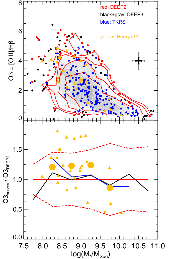
FIG. 2.— Upper : [\text{OIII}]/\text{H}\beta flux ratio as a function of M_* for galaxies in our sample. Galaxies from different surveys are shown by filled circles with different colors. The DEEP2 (and DEEP3) distribution is shown by red (and gray) contours plus red (and black) circles. The thick black (and thin gray) error bars show the median (and 90 percentile) of the 1\sigma uncertainty of the [\text{OIII}]/\text{H}\beta and M_* measurements. For comparison, data of H13 are shown as yellow triangles. Lower : sample-to-sample variation in the [\text{OIII}]/\text{H}\beta flux ratio. We use our DEEP2 sub-sample as a base sample and show the ratio between the average [\text{OIII}]/\text{H}\beta of other sub-samples and that of the base sample. The color scheme is the same as that in the upper panel. The base sample (DEEP2) is shown as a constant red solid line at unity, and its 1\sigma confidence level is shown by red dashed lines. H13 data are shown as yellow triangles, while their average values are shown as large yellow circles.
