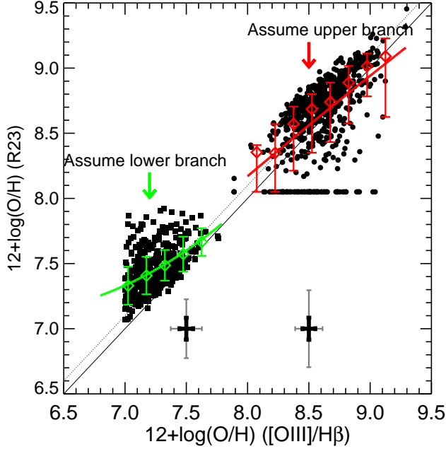
FIG. 3.— Comparison between metallicities measured by R23 and [\text{OIII}]/\text{H}\beta in the DEEP3 sample. Circles (the right locus) show the case of using the upper-branch metallicity values for all galaxies, while squares (the left locus) the lower-branch values. Red (green) diamonds and error bars show the median and 16 and 84 percentiles of the comparison for the upper (lower) branch case. The red (green) curve shows a second-order polynomial fit to the comparison of the upper (lower) branch case. The right and left black (gray) error bars show the median (90 percentile) measurement uncertainty of the upper and lower branches, respectively.
