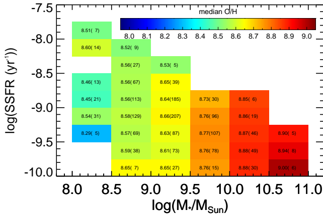
FIG. 6.— SSFR dependence of the MZR. The median metallicity of each ( M_* , SSFR) bin is shown by color, with the color bar in the upper right part. The median metallicity value as well as the number of galaxies in each bin are also given. Each bin spans 0.5 dex in M_* and 0.25 dex in SSFR.
