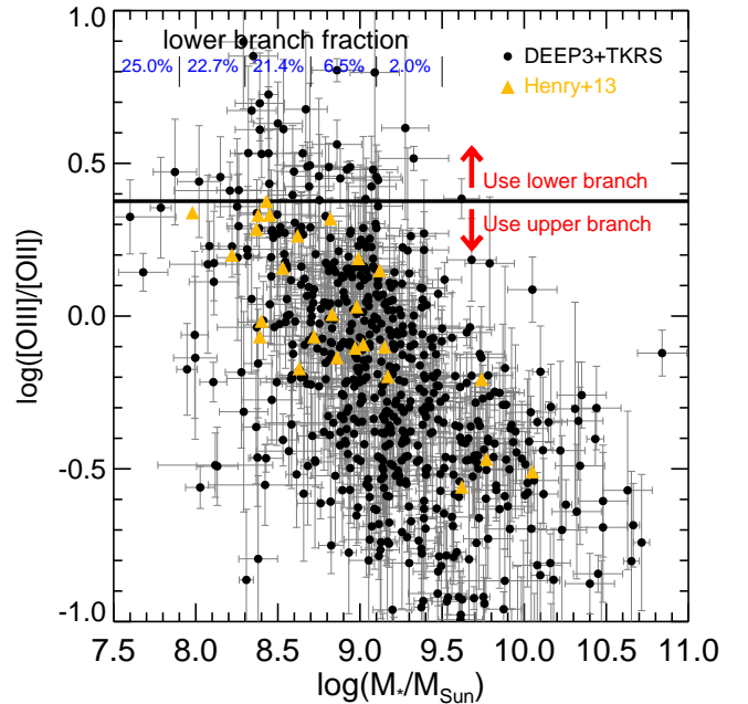
FIG. 4.— Using [\text{OIII}]/[\text{OII}] to break the lower-upper branch degeneracy in the DEEP3+TKRS training sample. Each black circle with gray error bars shows one galaxy. Galaxies above \log([\text{OIII}]/[\text{OII}]) = 0.375 (black horizontal line) are identified to use their lower-branch metallicities, and vice versa. In each mass bin (width of 0.4 dex), the fraction of galaxies in the lower branch is given by the blue number in top. For comparison, data of H13 are shown as yellow triangles.
