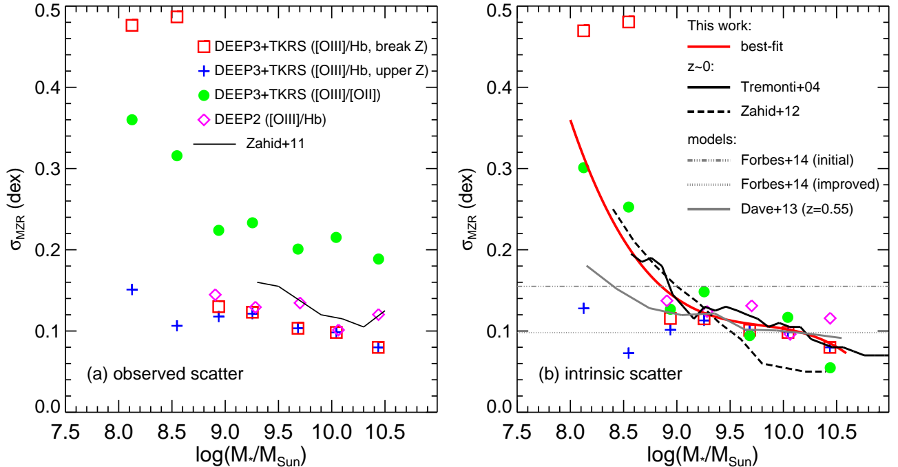
FIG. 7.— Scatter of the MZR of our sample. Scatter is defined as the half-width between the 84th and 16th percentiles ( P_{84} and P_{16} ) of the metallicity distribution at a given M_* . Left (a) : Observed scatter. Measurements from different samples and/or different methods of breaking the lower–upper branch degeneracy are plotted with different symbols as the labels show. We only measure the scatter of DEEP2 down to M_* = 10^9 M_{\odot} . The solid black line shows the scatter of Zahid et al. (2011) at z \sim 0.8 from DEEP2 data. Right (b) : Intrinsic scatter. The measurement uncertainties are subtracted from the observed scatter in quadrature. Symbols have the same meaning as in Panel (a). A third-order polynomial function is fitted to our measurements: red squares, green circles, and purple diamonds at M_* \geq 10^9 M_{\odot} and only green circles at M_* \leq 10^9 M_{\odot} . The scatter of local MZR of Tremonti et al. (2004) and Zahid et al. (2012) are shown by solid and dashed black lines. The scatter from the initial and improved guesses of Forbes et al. (2014b) are shown by dashed–dotted and dotted grey lines. The scatter of numerical simulations of Davé et al. (2013) is shown by the solid grey line.
