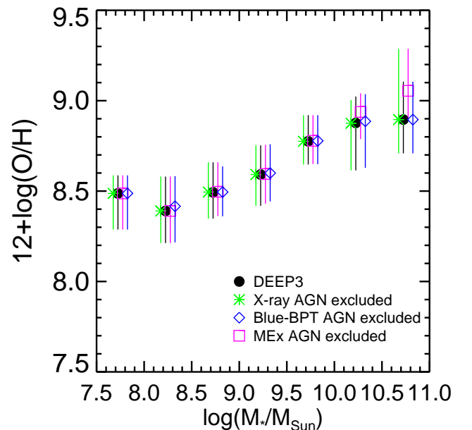
FIG. 10.— Effect of AGN removal on the MZR measurement. For simplicity, all galaxies are assumed to be in the upper branch, and no conversion uncertainty is included. Large black circles with error bars show DEEP3+TKRS galaxies without any AGN removal. MZRs with different AGN removal methods are shown by different symbols as indicated by the labels. The MEx method (purple squares) is the fiducial method used in our paper.
