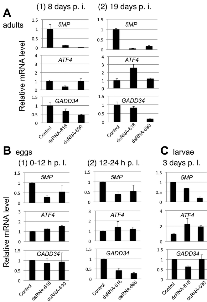
Figure 6. Effect of 5MP RNAi on expression of 5MP, ATF4 and GADD34 in T. castaneum . (A) Relative mRNA expression for 5MP (top), ATF4 (middle), and GADD34 (bottom) in beetles 8 (panel 1) and 19 (panel 2) days post-injection (p. i.) of two non-overlapping RNAi fragments (1 \mu\text{g}/\mu\text{l} ) directed to 5MP, termed 5MP dsRNA-616 or dsRNA-690. RNA abundance was quantified with qRT-PCR and presented as in Figure 5A and B. (B) Expression in eggs 0–12 h (panel 1) or 12–24 h (panel 2) post-lay (p. l.) by injected adults. In panel 1, 5MP, ATF4 and GADD34 expression normalized to RPS3 was examined right after the injected adults were allowed to lay eggs for 12 h and presented in values relative to expression from mock-treated adults. In panel 2, expression was similarly examined after the eggs collected similarly were aged for an additional 12 h. (C) 5MP, ATF4 and GADD34 expression normalized to RPS3 in larvae 3 days post-lay by injected adults. Presented are values relative to expression from mock-treated adults. In (B) and (C), the average of two biological replicates are shown with SEM.
