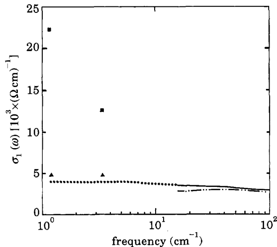
Fig. 4. - Optical conductivity of U_2Zn_{17} in the FIR frequency range at 300 (—) and 6 K (---) together with the measurements at 35 and 100 GHz: ■ at 6 K, ▲ at 300 K.
