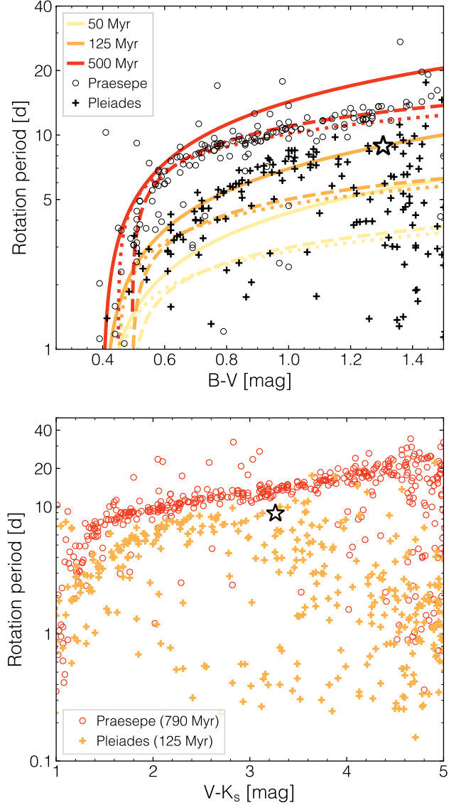
Figure 9. Top: Gyrochrones in the period versus ( B - V ) plane. The solid, dashed, and dotted lines show gyrochrones predicted from Barnes (2007), Mamajek & Hillenbrand (2008), and Angus et al. (2015), respectively. Bottom: Rotation periods versus ( V - K_s ) color for Praesepe (red) and Pleiades (orange) members. In both figures the cluster rotation periods are taken from Rebull et al. (2016, 2017) and the white star indicates K2-284.
