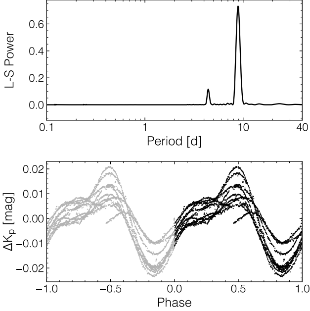
Figure 7. Lomb-Scargle periodogram from K2 photometry of K2-284 (top) and the light curve phased to the rotation period of 8.88 d (bottom).
