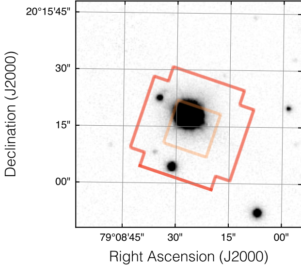
Figure 2. Pan-STARRS r -band image centered on K2-284 showing the adopted K2 aperture in red and a smaller aperture in orange, from which the transits were also recovered at a consistent depth. We also inspected photometry from 4'' wide square apertures centered on the neighboring stars to the south and to the east to confirm that neither are eclipsing binaries.
