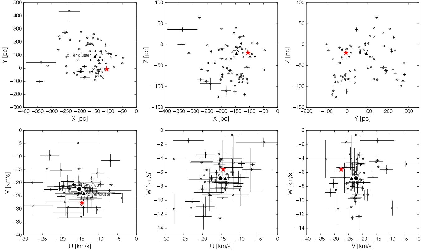
Figure 8. XYZ positions and UVW space motions for proposed Cas-Tau members (open circles; de Zeeuw et al. 1999), the \alpha Per cluster (filled triangle; based on the Gaia DR2 astrometry and radial velocity from Gaia Collaboration et al. 2018b), and K2-284 (red star). The errorbars reflect 1\sigma uncertainties for de Zeeuw et al. (1999) Cas-Tau members using Gaia DR2 parallaxes, combined with RVs from DR2 when available or de Bruijne & Eilers (2012) otherwise. In the bottom panels, the filled circle indicates the median velocity of the proposed Cas-Tau members, without outlier rejection. The cluster of points in the lower right of the first two panels is due to the newly identified \mu Tau group, which will be the subject of a future work.
