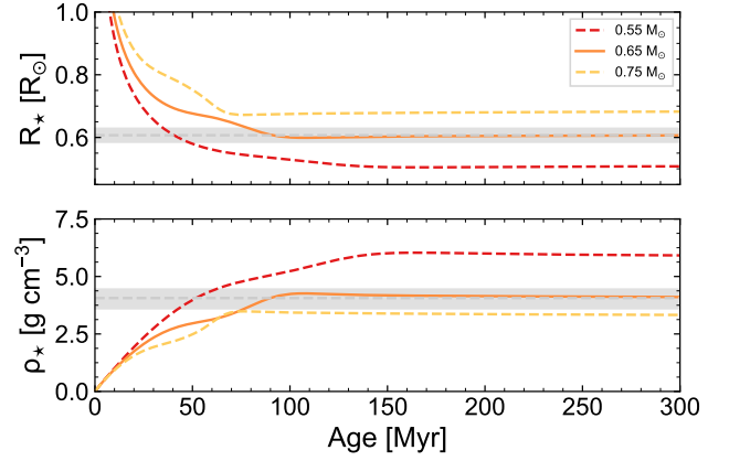
Figure 6. Theoretical predictions from the MIST models (Choi et al. 2016) of the evolution in radius (upper panel) and mean stellar density (lower panel) for low-mass stars. The grey lines and shaded regions show the adopted stellar radius and the mean stellar density measured from the transit fit.
