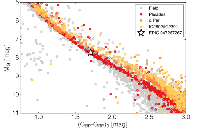
Figure 14. Color-absolute magnitude diagram for K2-284 as well as young cluster members and field stars, for comparison. K2-284 is apparently on the main sequence, with an age that is likely older than \alpha Per, IC 2602, or IC 2391, but consistent with the locations of Pleiades members and field stars.
