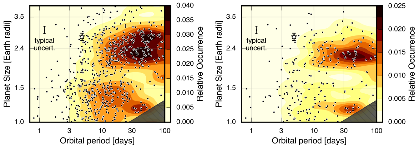
Figure 15. The distribution of small transiting planets in the plane of planet radius and orbital period for the full California-Kepler Survey sample, at left, and only “low-mass” hosts ( < 0.97 M_{\odot} ) at right. K2-284 b is indicated by the white star. Overlaid are contours of completeness-corrected occurrence rates (Fulton et al. 2017; Fulton & Petigura 2018).
