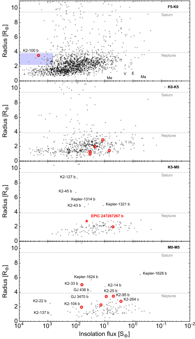
Figure 16. The distribution of confirmed, small transiting planets from the NASA Exoplanet Archive (Akeson et al. 2013) in the plane of planet radius and insolation flux. Planets transiting stars in clusters or associations are circled in red. K2-284 b is indicated by the red star. Each panel corresponds to a different range in host star spectral type (annotated at top right). K2-284 b is on the larger end of known, close-in sub-Neptunes around stars of a similar spectral type. A number of other planets orbiting cool young cluster stars also appear to be anomalously large. The blue region in the top panel indicates the hot planet desert described in Lundkvist et al. (2016).
