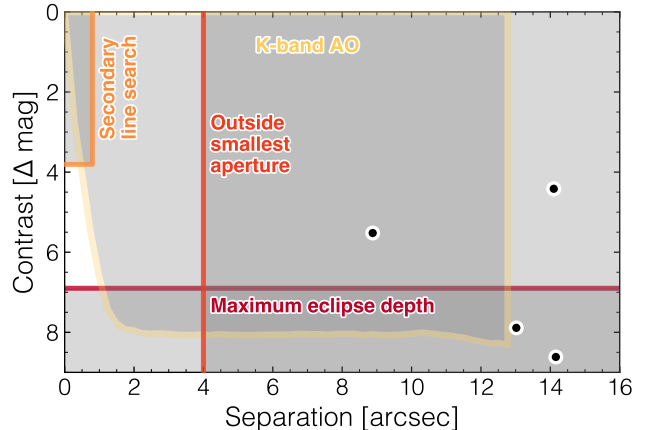
Figure 4. Contrast versus projected angular separation. The grey shaded regions show the excluded areas of parameter space in which a putative false positive could reside. The black points show nearby sources detected by Pan-STARRS. Note the secondary line search is blind to companions with velocity separations <15 \text{ km s}^{-1} from the primary.
