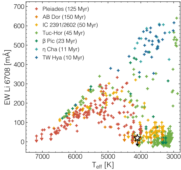
Figure 11. Li I 6708 Å equivalent width versus T_{\text{eff}} for members of Pleiades ( Soderblom et al. 1993 ), IC 2391/2602 ( Randich et al. 2001 ), and young moving groups ( Mentuch et al. 2008 ; Kraus et al. 2014 ). K2-284 is indicated by the white star.
