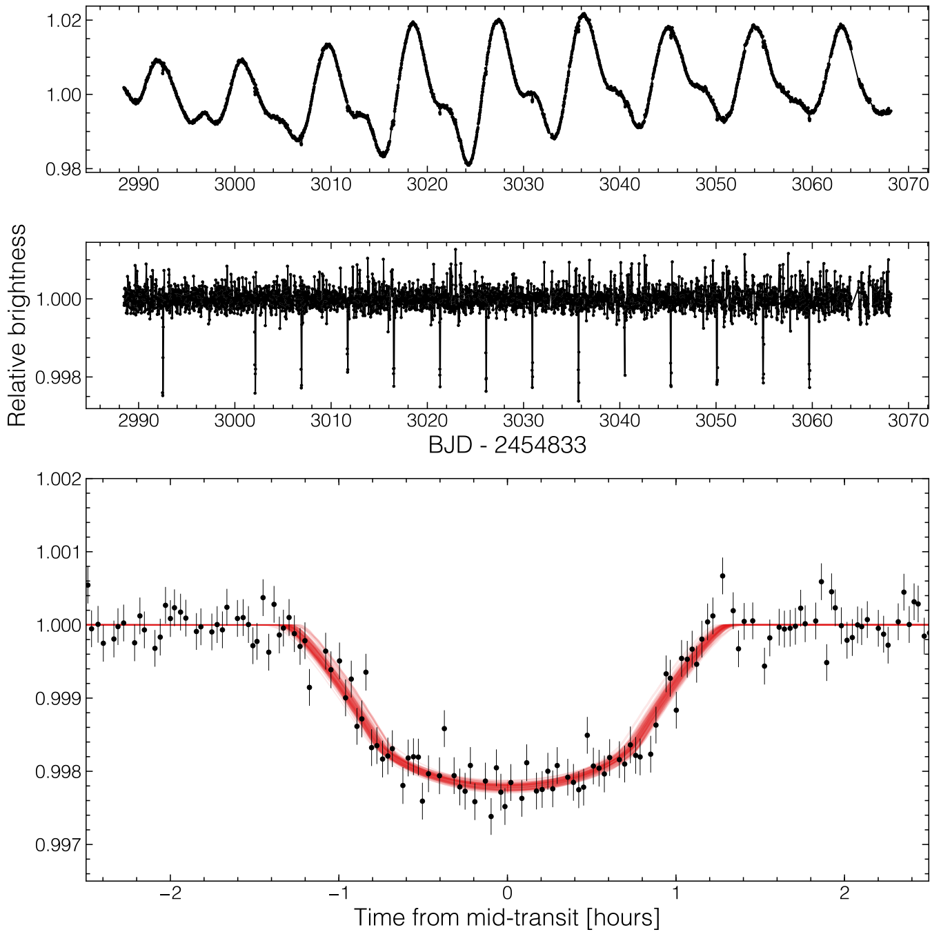
Figure 1. K2 light curve of K2-284. In the top panel, the stellar variability pattern due to rotational modulation of starspots is apparent, as are the transits of K2-284 b. In the middle panel, the stellar variability has been removed. Missing transits are due to sections of the light curve that were removed in the detrending procedure. In the bottom panel, phase-folded model fits to the transits of K2-284 b. The red curves show 200 randomly selected models from the MCMC chain.
