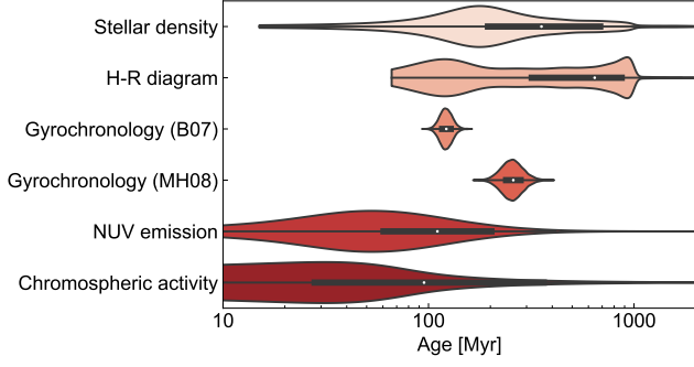
Figure 13. Violin plot demonstrating the kernel density estimates for stellar age distributions resulting from different age-dating methods discussed in § 3.5.
