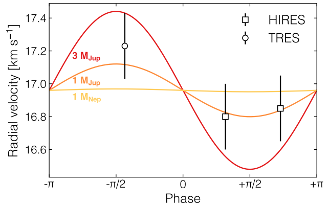
Figure 5. Radial velocities phased to the orbital ephemeris of K2-284 b. We find no evidence for orbital motion and from these measurements place an upper limit to the planet’s mass of < 3 M_{\text{Jup}} at 95% confidence. The expected RV curves for planet masses corresponding to Neptune, Jupiter, and three times the mass of Jupiter are shown by the colored curves.
