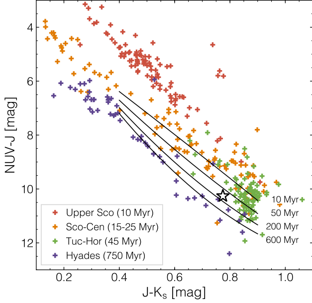
Figure 10. NUV and NIR color-color diagram showing empirical isochrones of Findeisen et al. (2011) and members of young stellar populations. K2-284 is indicated by the white star.
