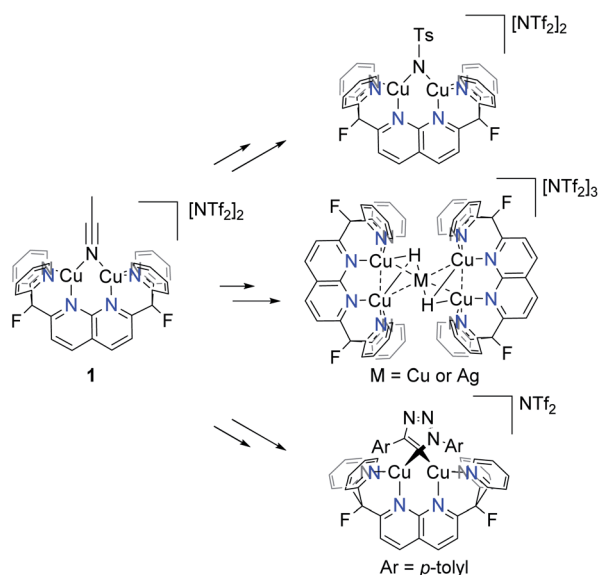
Scheme 2 Examples of detected and/or isolated reactive intermediates containing the [(DPFN)Cu 2 ] + scaffold.
