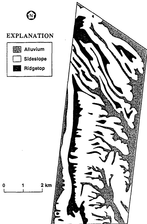
Fig.5 Approximate view of the different infiltration zones used in the site-scale model.
