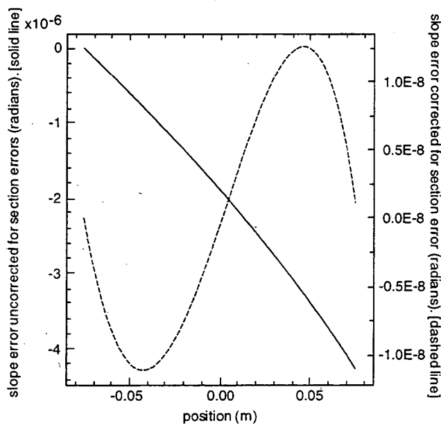
Fig. 8. Solid line shows the figure error resulting from a constant width error of 0.2 mm. Dotted line shows the minimization of the error by adjustment of C_1 and C_2 .
