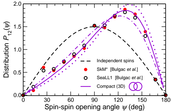
FIG. 3: The opening-angle distributions calculated by Bulgac et al. [6] with time-dependent density functional theory using either the SkM* or the SeaLL1 energy density functional are compared with 3D sampling results for a compact scenario for which \mathcal{I}_1 : \mathcal{I}_2 : \mathcal{I}_0 = 1 : 1 : 2 . To illustrate the sensitivity to \mathcal{I}_0 are also shown the distributions for a 50% smaller (dots) or a 50% larger (dot-dash) \mathcal{I}_0 value.
