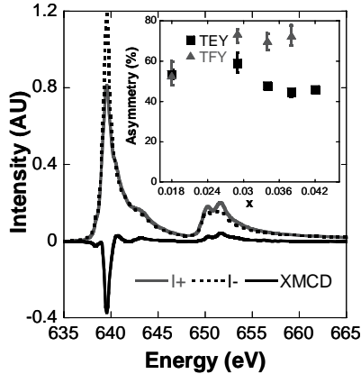
FIGURE 1. (main) Mn L 3,2 TEY XAS spectra for magnetization and helicity parallel (I + ) and antiparallel (I - ) as well as the difference (XMCD) spectrum for a Ga 1-x Mn x P sample with x=0.034 measured at 17 K. (inset) TEY and TFY asymmetry at the Mn L 3 peak versus x.
