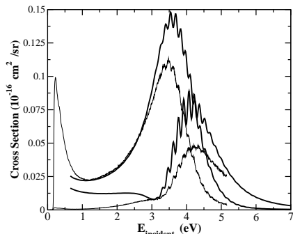
Figure 3. Differential vibrational excitation cross sections at 135^\circ for upper and lower members of the Fermi dyad in \text{CO}_2 . Thick solid curves were calculated and thin solid curves are experimental results of Allan ([3]).
