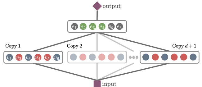
Figure 4: Schematic of the padding strategy to prove Theorems 7-8.
