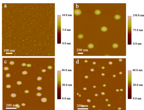
Figure 2. AFM images of YMA (a) and DNA hydrogel nanoparticles with different molar ratios of YMA to YMB: (b) 4:1 (NP-1), (c) 3:1 (NP-2), (d) 2:1 (NP-3).
