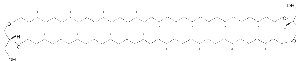
(g) Diradylglycerols: Di-glycerol tetraethers: caldarchaeol
