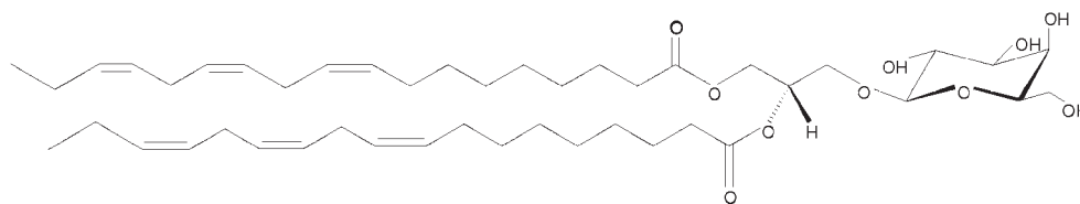
(f) Diradylglycerols: Diacylglycerol glycans: 1,2 di-(9Z,12Z,15Z-octadecatrienoyl)-3-O-β-D-galactosyl- sn -glycerol
