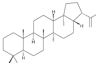
(o) Hopanoids: diplotene; hop-22(29)-ene
