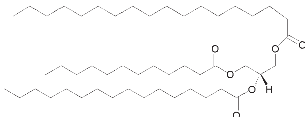
(e) Triradylglycerols: Tricylglycerols: 1-dodecanoyl-2-hexadecanoyl-3-octadecanoyl- sn -glycerol
