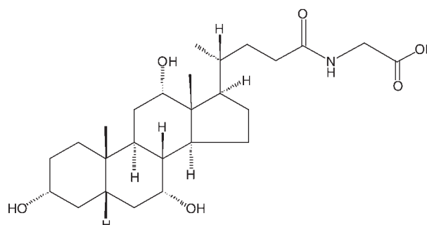
(m) Steroid conjugates: Glycine conjugates: glycocholic acid; N-(3 \alpha ,7 \alpha ,12 \alpha -trihydroxy-5 \beta - cholan-24-oyl)-glycine
