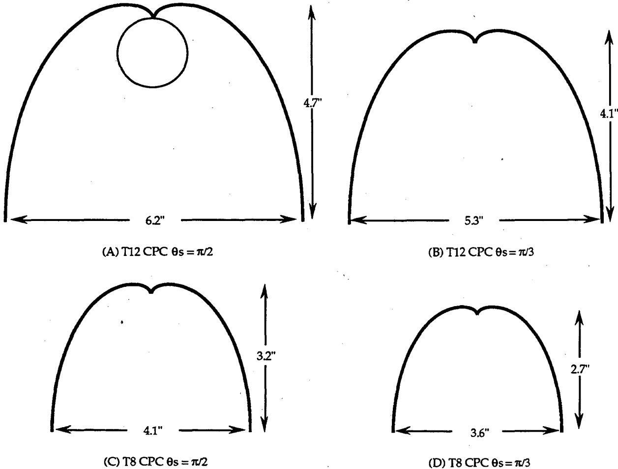
Fig. 3. CPC reflector profiles with cutoff angles of 50^\circ for cylindrical fluorescent lamps of different size and values of \theta_s .
