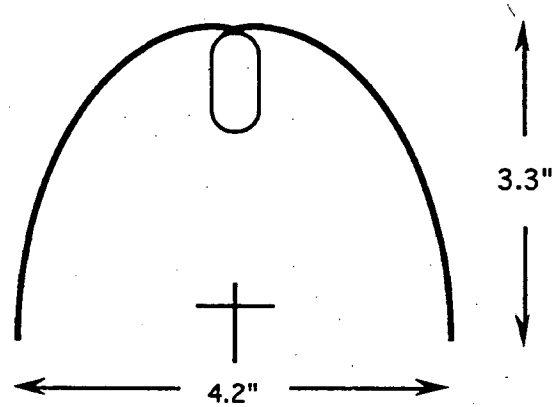
(C) Cross-sectional view of CPC reflector troffer for a twin tube CFL.
