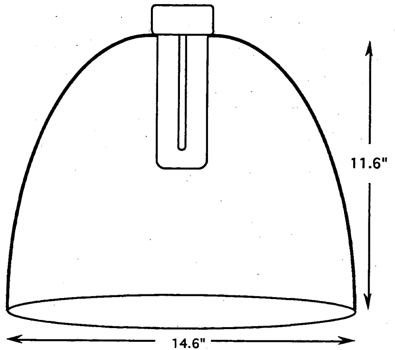
(D) Cross-sectional view of CPC reflector spinner for a twin tube CFL.
