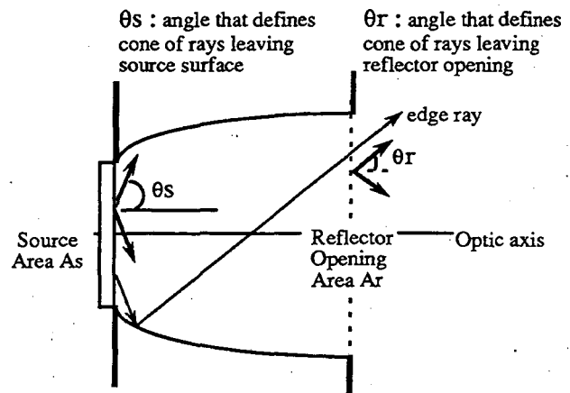
Fig. 1. Flux that leaves any point on a source area A_S within an angle \theta_S can fully exit a reflector area A_R at an angle \theta_R or less provided (1) is satisfied.
