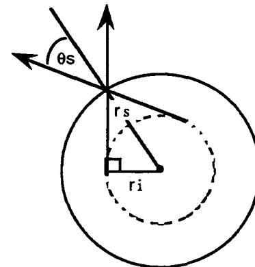
Geometrical relationship between a real and imaginary source. Rays leaving the real source within \theta_s can be considered to have left the smaller imaginary source tangentially.
