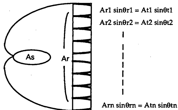
Fig. 5. CPC louver based on flux conservation. Each louver element may have its own shape and orientation to meet geometric task requirements.
